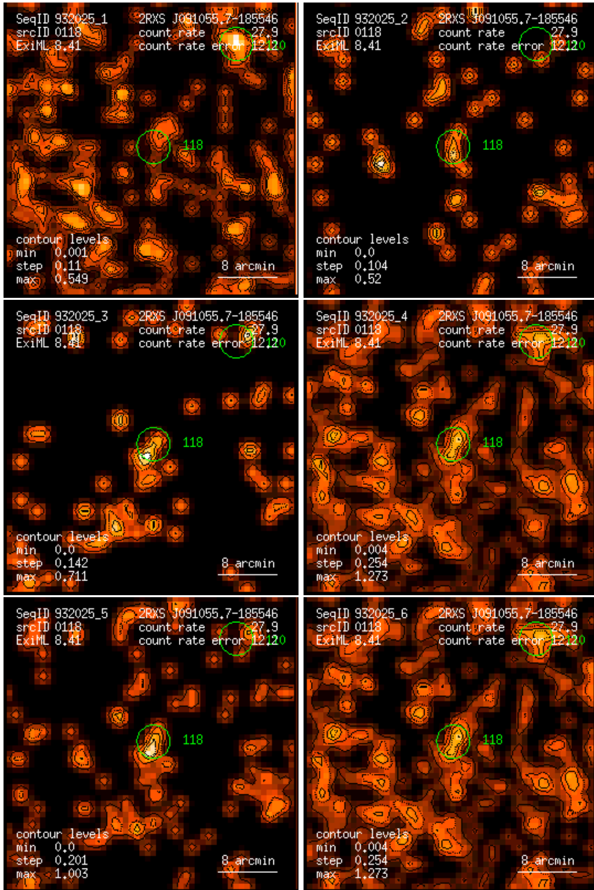
Figure 118: RASS 932025: detection 0118: band rate images, Gaussian filter: (1) PSPC channels 11 – 41, (2) 52 – 90, (3) 91 – 201, (4) 11 – 235, (5) 52 – 201, (6) 11 – 201. Broad band rates in counts/ks. Band rate contour levels in counts/ks/arcmin 2 .
