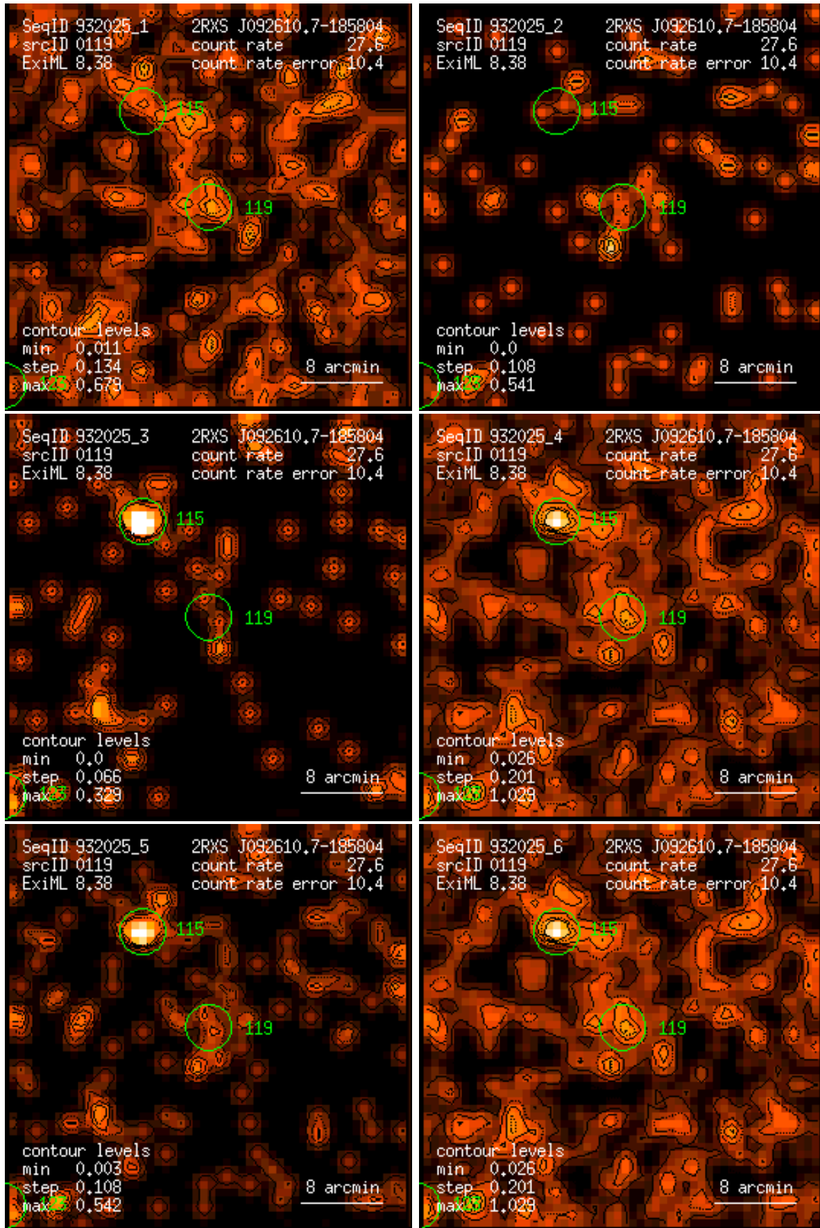
Figure 119: RASS 932025: detection 0119: band rate images, Gaussian filter: (1) PSPC channels 11 – 41, (2) 52 – 90, (3) 91 – 201, (4) 11 – 235, (5) 52 – 201, (6) 11 – 201. Broad band rates in counts/ks. Band rate contour levels in counts/ks/arcmin 2 .
