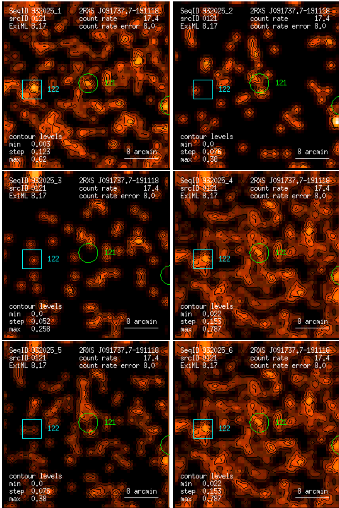
Figure 121: RASS 932025: detection 0121: band rate images, Gaussian filter: (1) PSPC channels 11 – 41, (2) 52 – 90, (3) 91 – 201, (4) 11 – 235, (5) 52 – 201, (6) 11 – 201. Broad band rates in counts/ks. Band rate contour levels in counts/ks/arcmin 2 .
