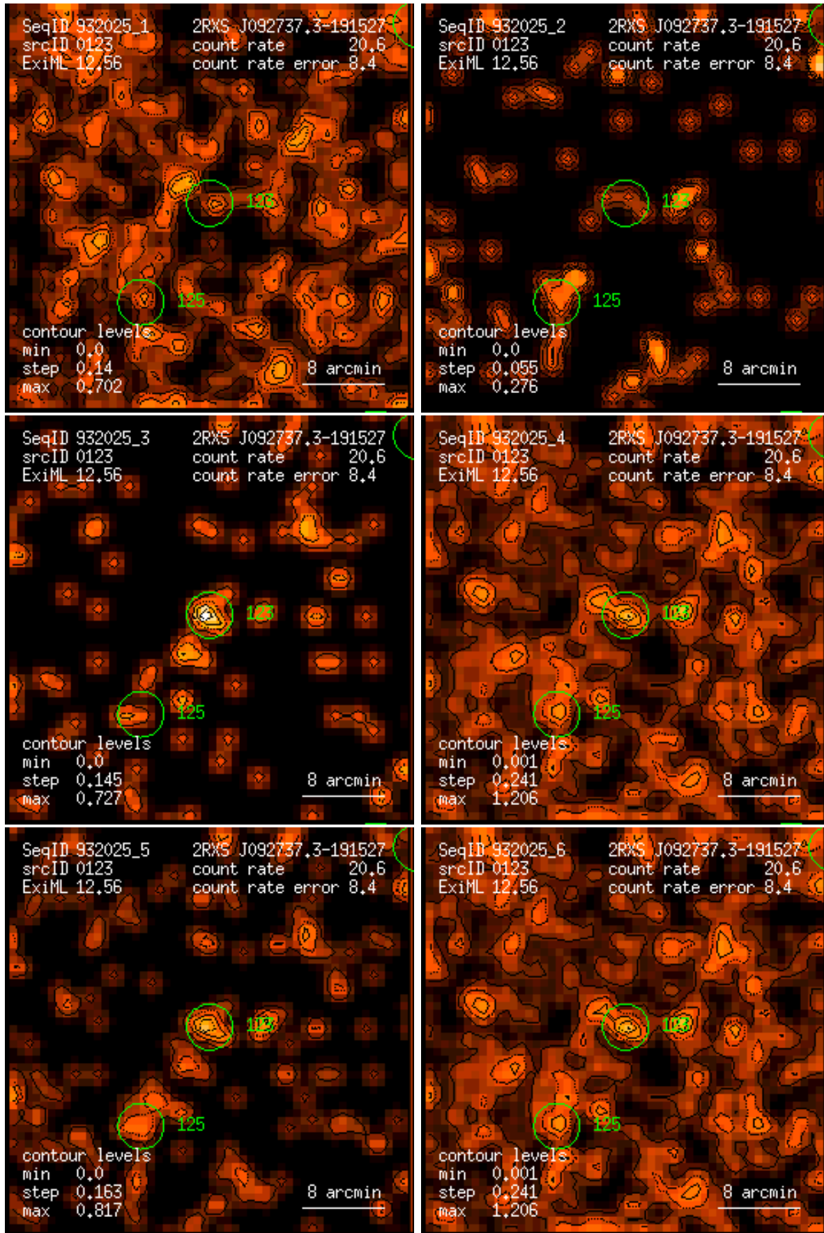
Figure 123: RASS 932025: detection 0123: band rate images, Gaussian filter: (1) PSPC channels 11 – 41, (2) 52 – 90, (3) 91 – 201, (4) 11 – 235, (5) 52 – 201, (6) 11 – 201. Broad band rates in counts/ks. Band rate contour levels in counts/ks/arcmin 2 .
