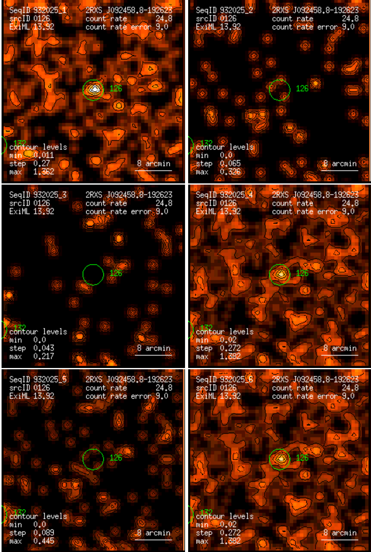
Figure 126: RASS 932025: detection 0126: band rate images, Gaussian filter: (1) PSPC channels 11 – 41, (2) 52 – 90, (3) 91 – 201, (4) 11 – 235, (5) 52 – 201, (6) 11 – 201. Broad band rates in counts/ks. Band rate contour levels in counts/ks/arcmin 2 .
