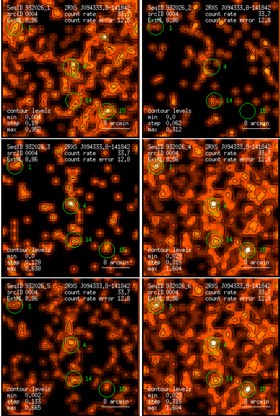
Figure 4: RASS 932026: detection 0004: band rate images, Gaussian filter: (1) PSPC channels 11 – 41, (2) 52 – 90, (3) 91 – 201, (4) 11 – 235, (5) 52 – 201, (6) 11 – 201. Broad band rates in counts/ks. Band rate contour levels in counts/ks/arcmin 2 .
