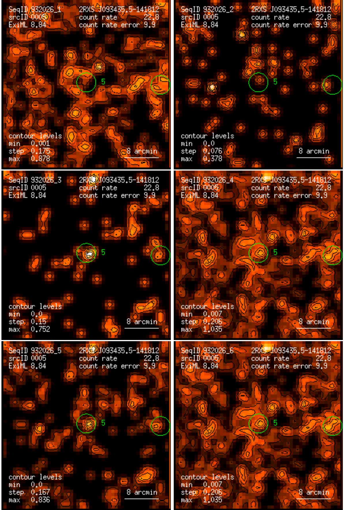
Figure 5: RASS 932026: detection 0005: band rate images, Gaussian filter: (1) PSPC channels 11 – 41, (2) 52 – 90, (3) 91 – 201, (4) 11 – 235, (5) 52 – 201, (6) 11 – 201. Broad band rates in counts/ks. Band rate contour levels in counts/ks/arcmin 2 .
