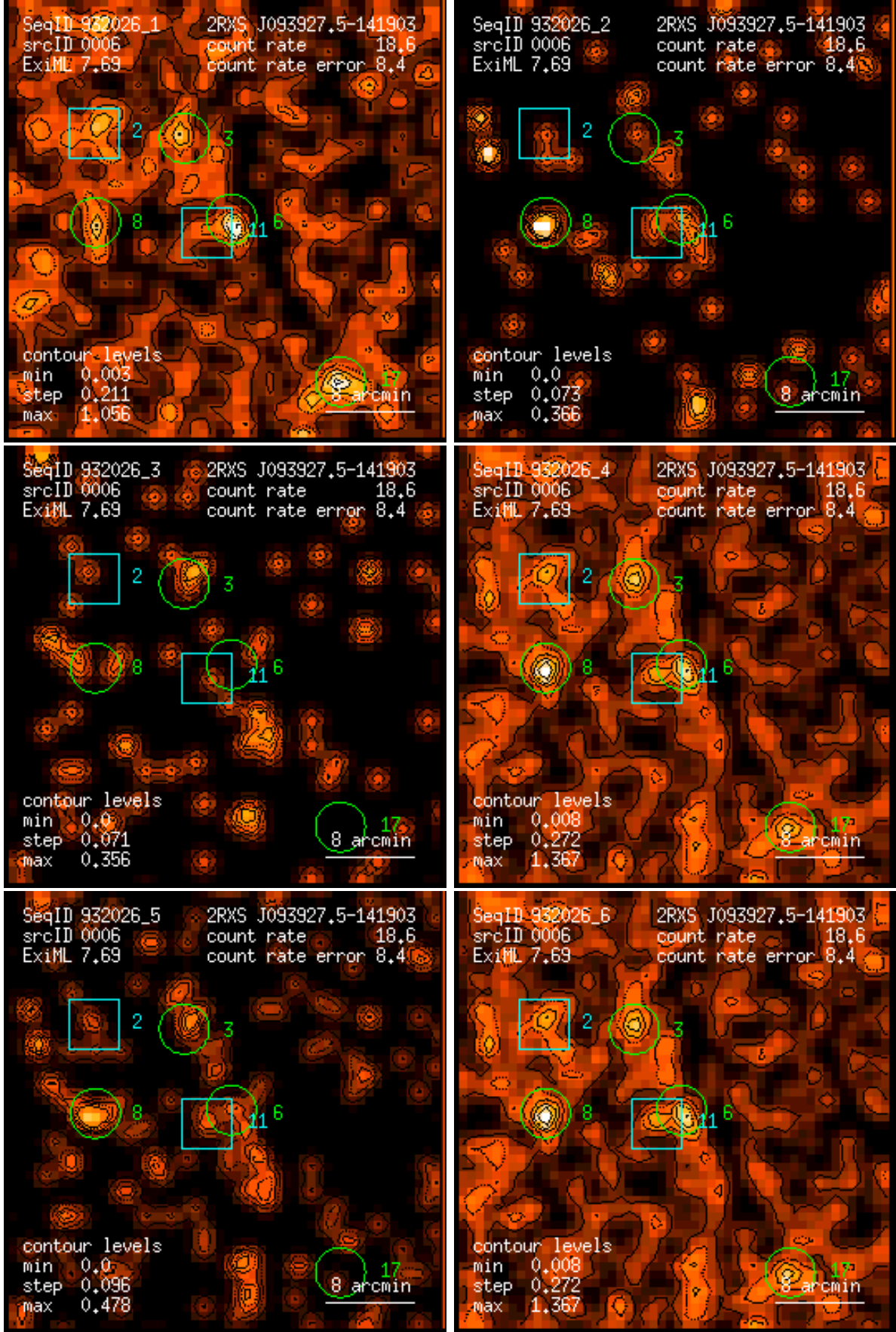
Figure 6: RASS 932026: detection 0006: band rate images, Gaussian filter: (1) PSPC channels 11 – 41, (2) 52 – 90, (3) 91 – 201, (4) 11 – 235, (5) 52 – 201, (6) 11 – 201. Broad band rates in counts/ks. Band rate contour levels in counts/ks/arcmin 2 .
