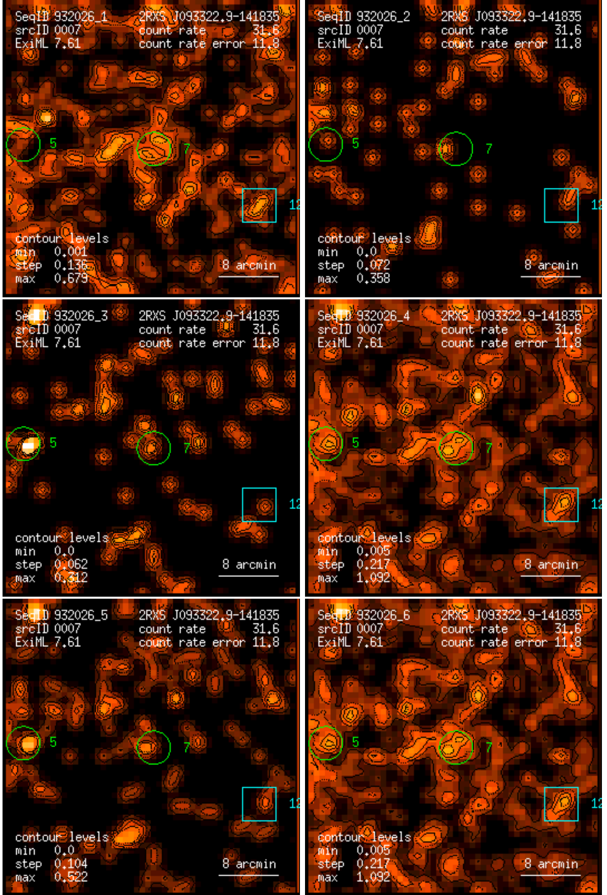
Figure 7: RASS 932026: detection 0007: band rate images, Gaussian filter: (1) PSPC channels 11 – 41, (2) 52 – 90, (3) 91 – 201, (4) 11 – 235, (5) 52 – 201, (6) 11 – 201. Broad band rates in counts/ks. Band rate contour levels in counts/ks/arcmin 2 .
