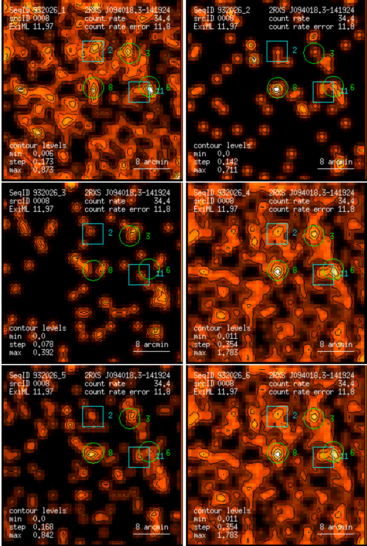
Figure 8: RASS 932026: detection 0008: band rate images, Gaussian filter: (1) PSPC channels 11 – 41, (2) 52 – 90, (3) 91 – 201, (4) 11 – 235, (5) 52 – 201, (6) 11 – 201. Broad band rates in counts/ks. Band rate contour levels in counts/ks/arcmin 2 .
