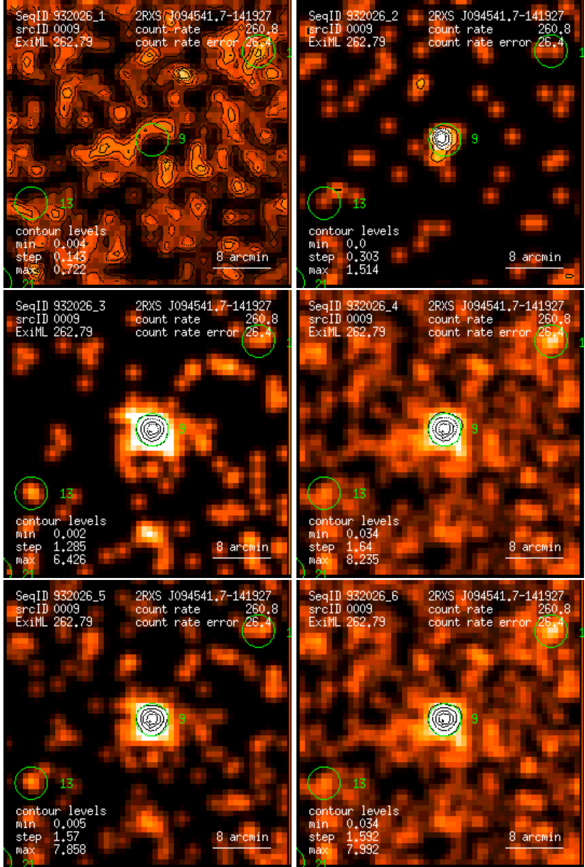
Figure 9: RASS 932026: detection 0009: band rate images, Gaussian filter: (1) PSPC channels 11 – 41, (2) 52 – 90, (3) 91 – 201, (4) 11 – 235, (5) 52 – 201, (6) 11 – 201. Broad band rates in counts/ks. Band rate contour levels in counts/ks/arcmin 2 .
