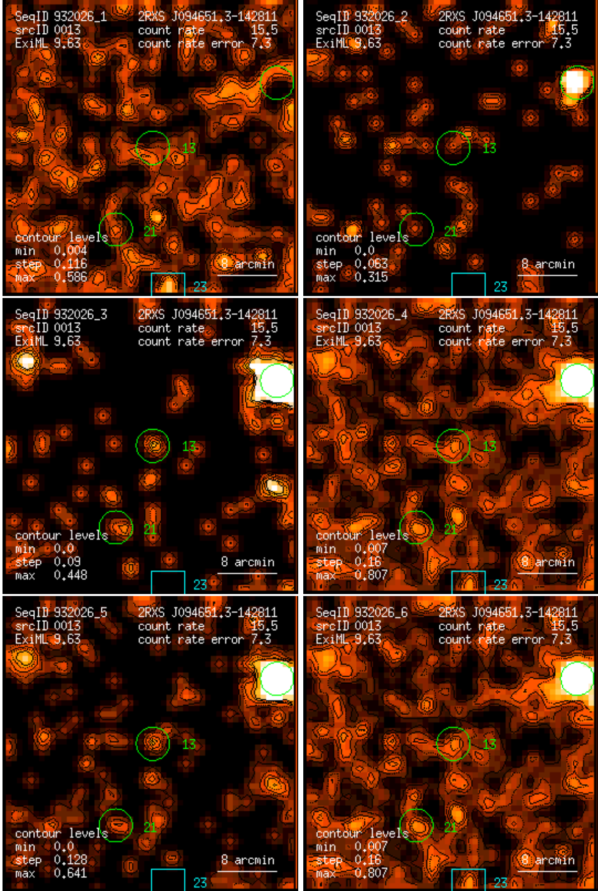
Figure 13: RASS 932026: detection 0013: band rate images, Gaussian filter: (1) PSPC channels 11 – 41, (2) 52 – 90, (3) 91 – 201, (4) 11 – 235, (5) 52 – 201, (6) 11 – 201. Broad band rates in counts/ks. Band rate contour levels in counts/ks/arcmin 2 .
