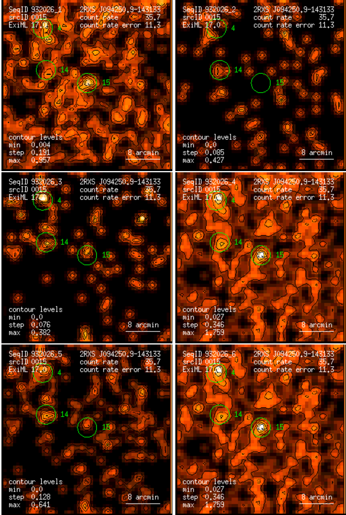
Figure 15: RASS 932026: detection 0015: band rate images, Gaussian filter: (1) PSPC channels 11 – 41, (2) 52 – 90, (3) 91 – 201, (4) 11 – 235, (5) 52 – 201, (6) 11 – 201. Broad band rates in counts/ks. Band rate contour levels in counts/ks/arcmin 2 .
