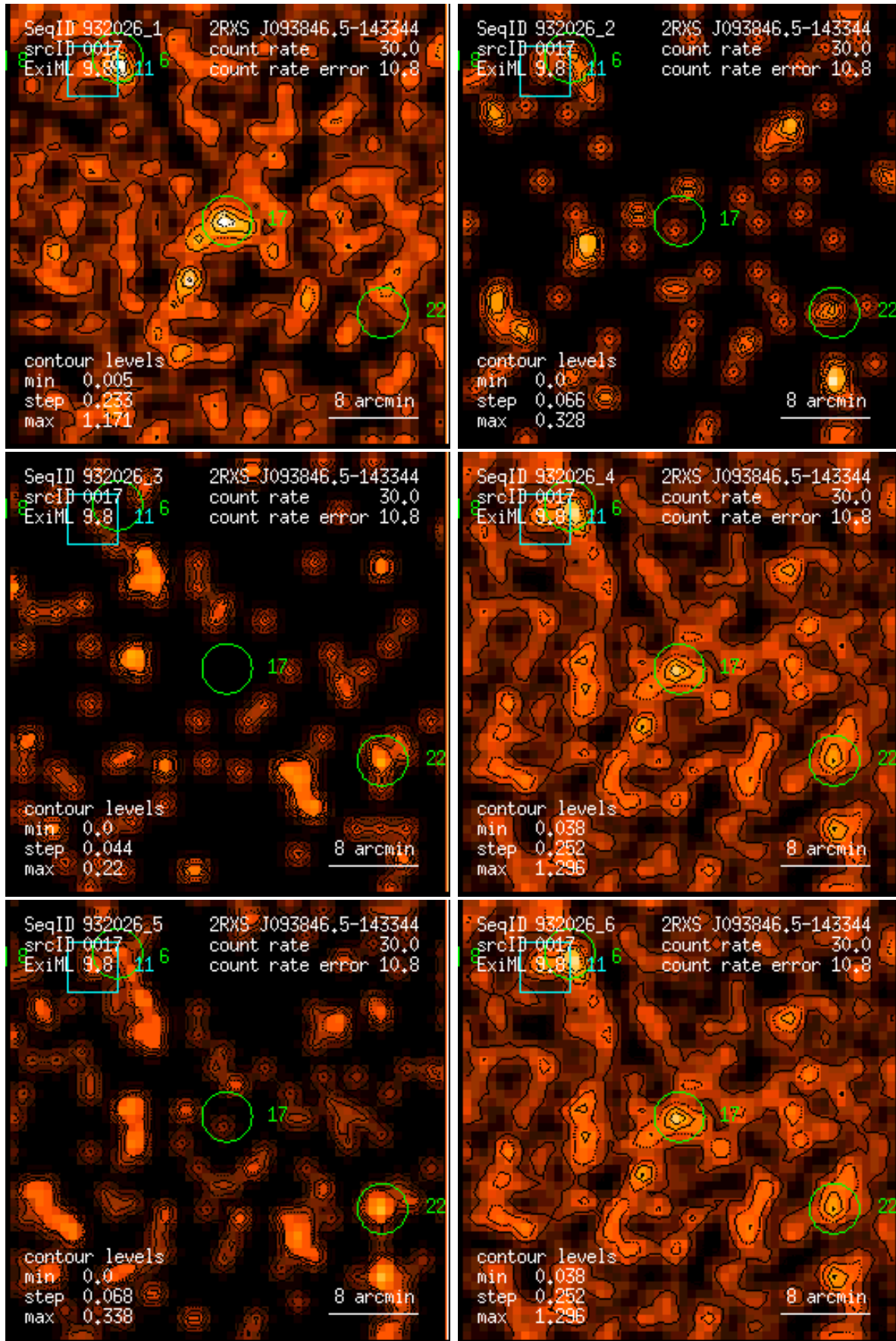
Figure 17: RASS 932026: detection 0017: band rate images, Gaussian filter: (1) PSPC channels 11 – 41, (2) 52 – 90, (3) 91 – 201, (4) 11 – 235, (5) 52 – 201, (6) 11 – 201. Broad band rates in counts/ks. Band rate contour levels in counts/ks/arcmin 2 .
