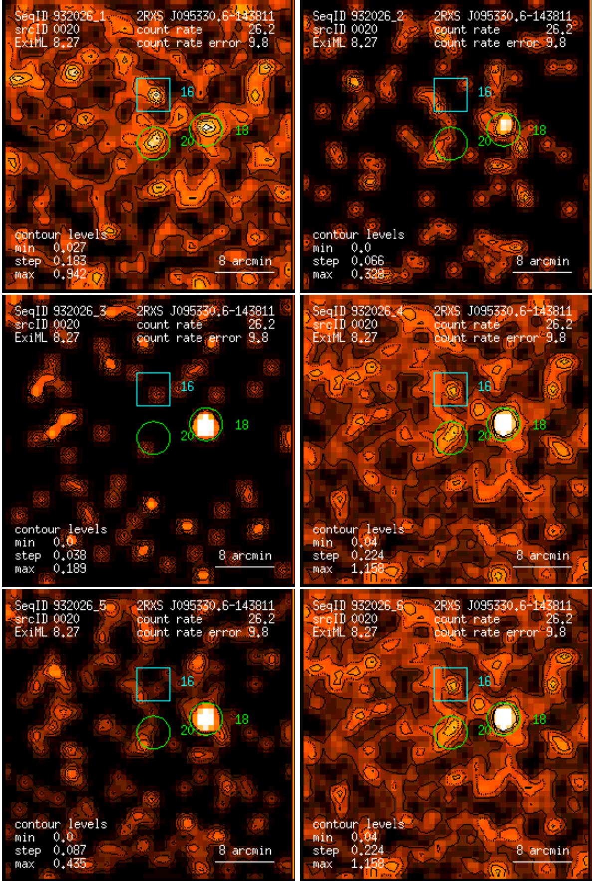
Figure 20: RASS 932026: detection 0020: band rate images, Gaussian filter: (1) PSPC channels 11 – 41, (2) 52 – 90, (3) 91 – 201, (4) 11 – 235, (5) 52 – 201, (6) 11 – 201. Broad band rates in counts/ks. Band rate contour levels in counts/ks/arcmin 2 .
