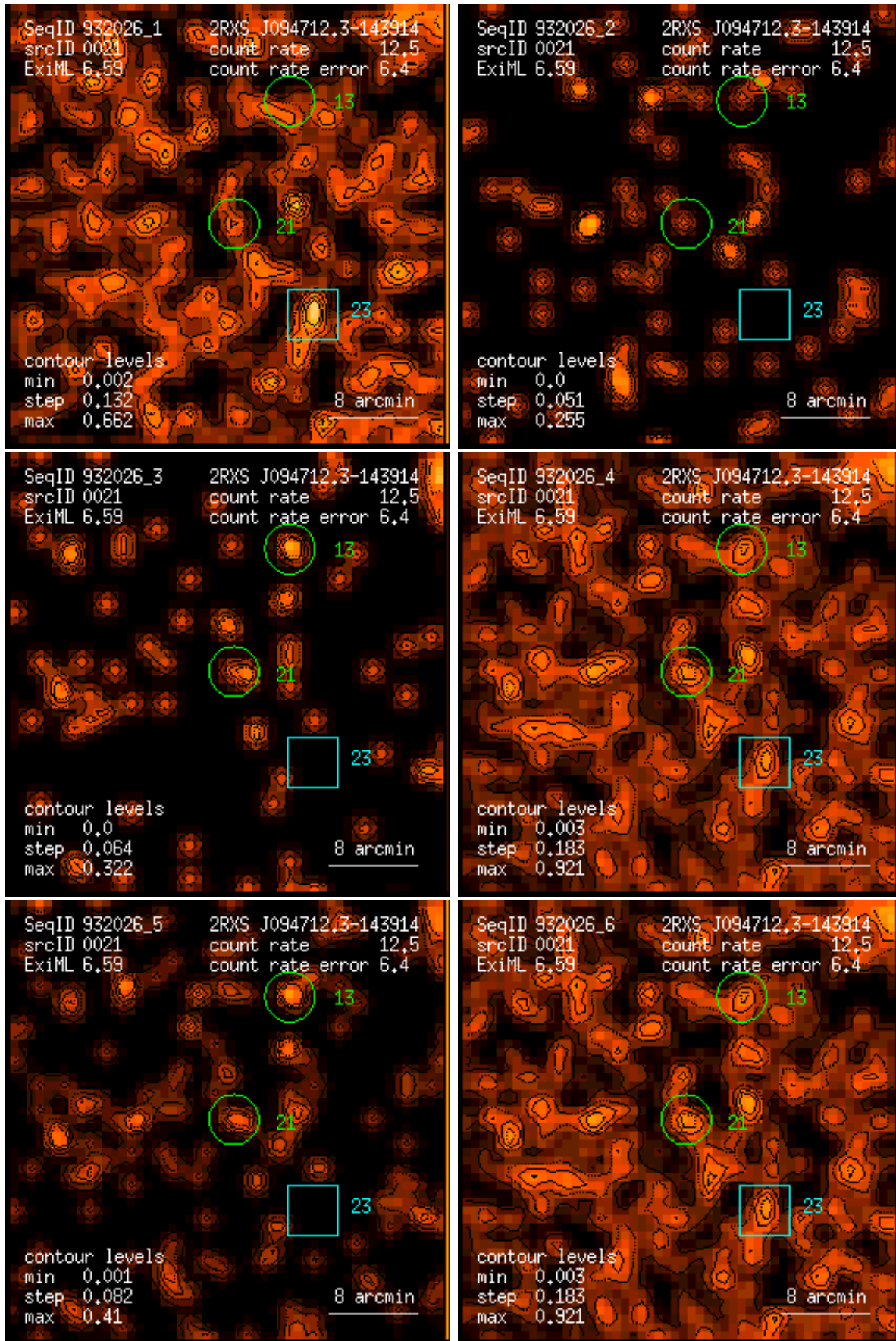
Figure 21: RASS 932026: detection 0021: band rate images, Gaussian filter: (1) PSPC channels 11 – 41, (2) 52 – 90, (3) 91 – 201, (4) 11 – 235, (5) 52 – 201, (6) 11 – 201. Broad band rates in counts/ks. Band rate contour levels in counts/ks/arcmin 2 .
