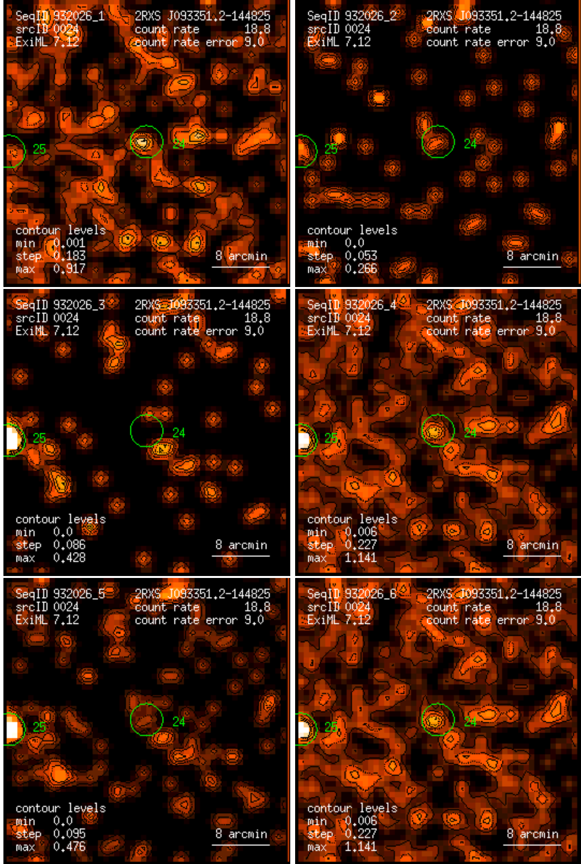
Figure 24: RASS 932026: detection 0024: band rate images, Gaussian filter: (1) PSPC channels 11 – 41, (2) 52 – 90, (3) 91 – 201, (4) 11 – 235, (5) 52 – 201, (6) 11 – 201. Broad band rates in counts/ks. Band rate contour levels in counts/ks/arcmin 2 .
