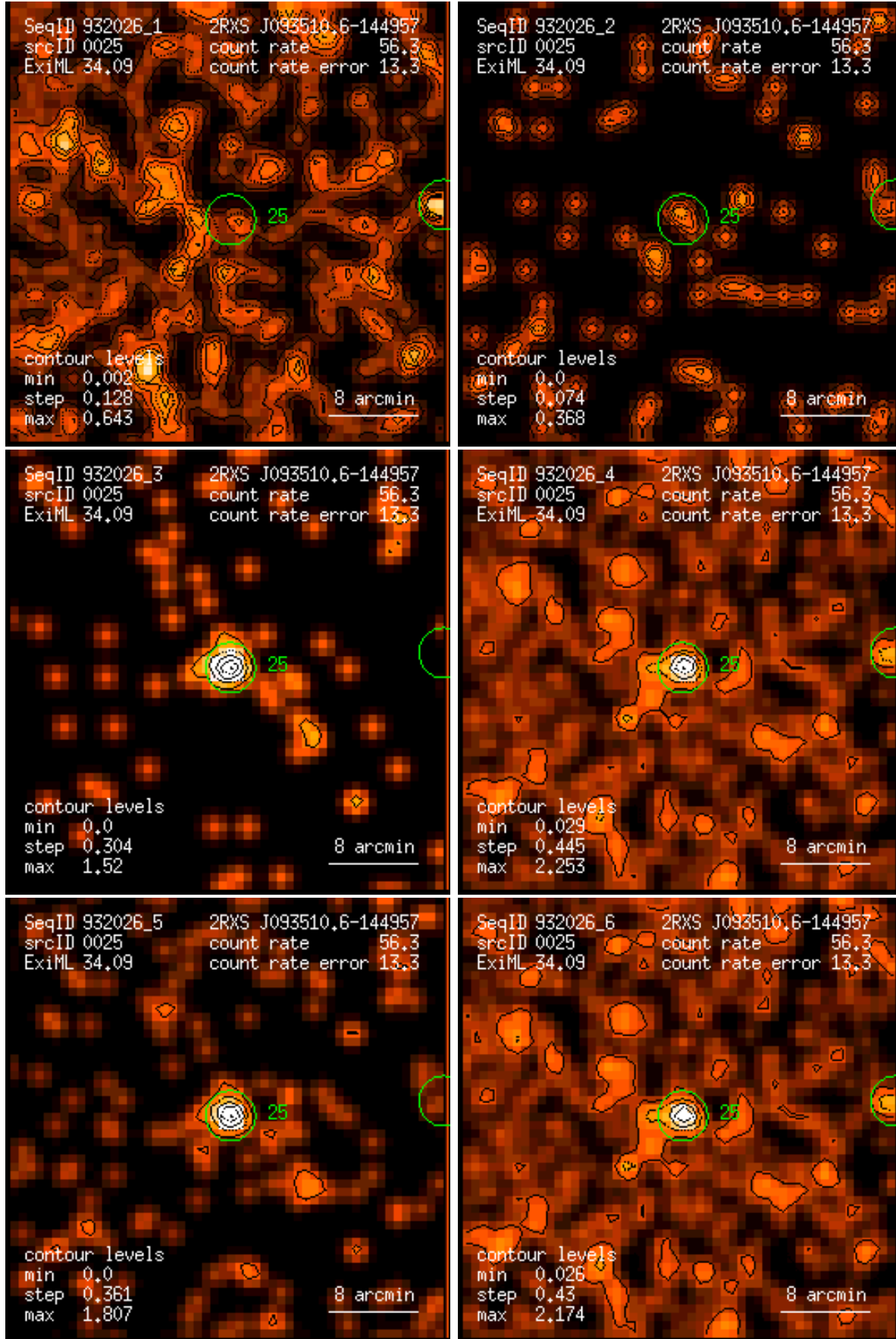
Figure 25: RASS 932026: detection 0025: band rate images, Gaussian filter: (1) PSPC channels 11 – 41, (2) 52 – 90, (3) 91 – 201, (4) 11 – 235, (5) 52 – 201, (6) 11 – 201. Broad band rates in counts/ks. Band rate contour levels in counts/ks/arcmin 2 .
