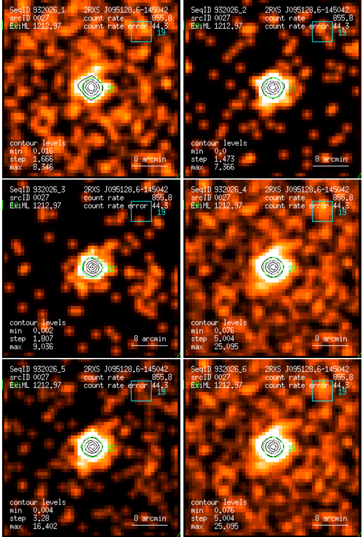
Figure 27: RASS 932026: detection 0027: band rate images, Gaussian filter: (1) PSPC channels 11 – 41, (2) 52 – 90, (3) 91 – 201, (4) 11 – 235, (5) 52 – 201, (6) 11 – 201. Broad band rates in counts/ks. Band rate contour levels in counts/ks/arcmin 2 .
