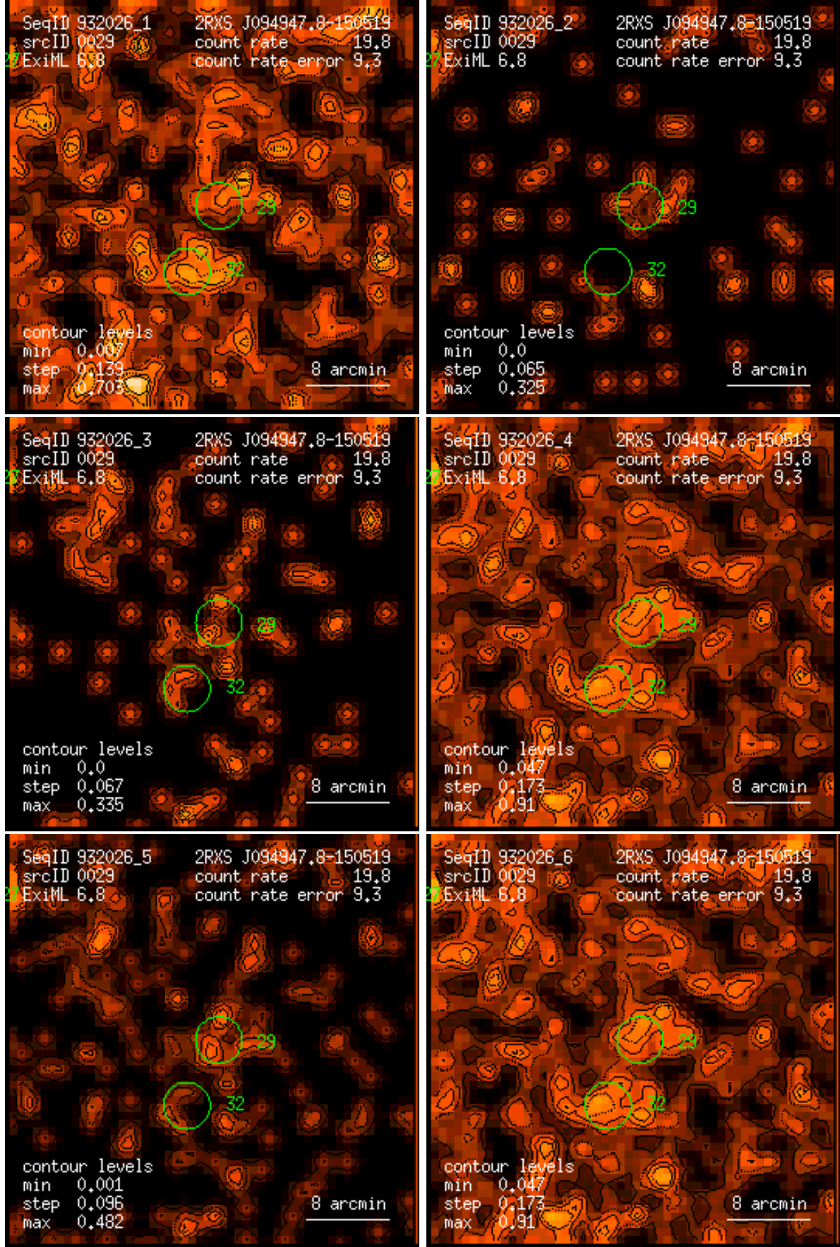
Figure 29: RASS 932026: detection 0029: band rate images, Gaussian filter: (1) PSPC channels 11 – 41, (2) 52 – 90, (3) 91 – 201, (4) 11 – 235, (5) 52 – 201, (6) 11 – 201. Broad band rates in counts/ks. Band rate contour levels in counts/ks/arcmin 2 .
