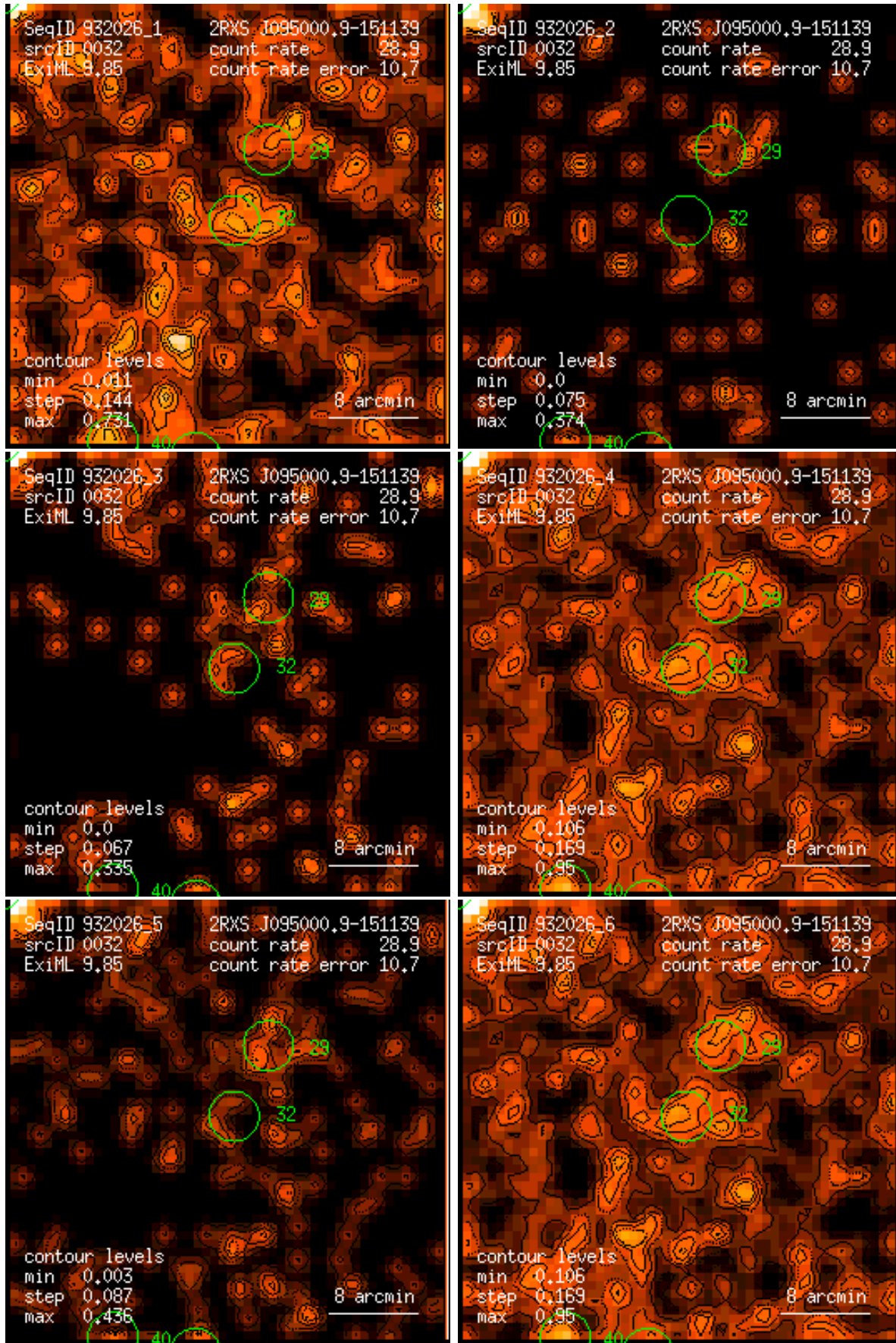
Figure 32: RASS 932026: detection 0032: band rate images, Gaussian filter: (1) PSPC channels 11 – 41, (2) 52 – 90, (3) 91 – 201, (4) 11 – 235, (5) 52 – 201, (6) 11 – 201. Broad band rates in counts/ks. Band rate contour levels in counts/ks/arcmin 2 .
