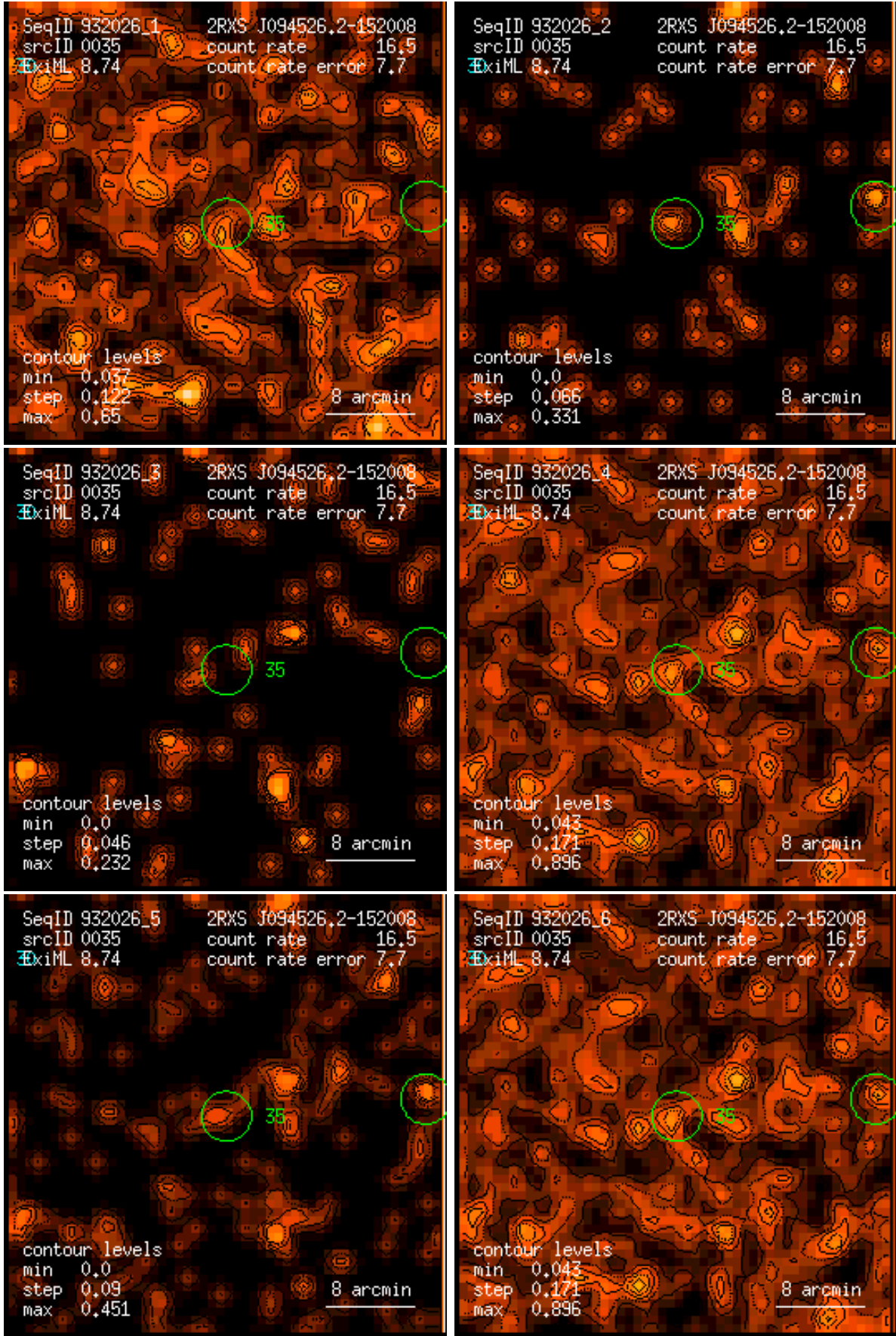
Figure 35: RASS 932026: detection 0035: band rate images, Gaussian filter: (1) PSPC channels 11 – 41, (2) 52 – 90, (3) 91 – 201, (4) 11 – 235, (5) 52 – 201, (6) 11 – 201. Broad band rates in counts/ks. Band rate contour levels in counts/ks/arcmin 2 .
