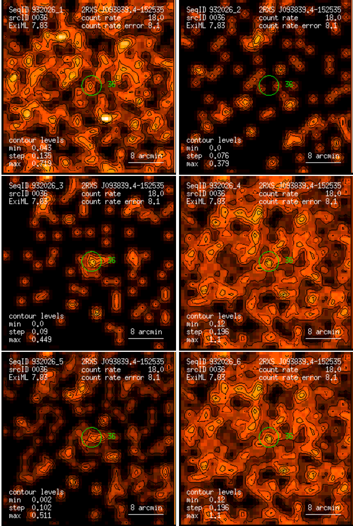
Figure 36: RASS 932026: detection 0036: band rate images, Gaussian filter: (1) PSPC channels 11 – 41, (2) 52 – 90, (3) 91 – 201, (4) 11 – 235, (5) 52 – 201, (6) 11 – 201. Broad band rates in counts/ks. Band rate contour levels in counts/ks/arcmin 2 .
