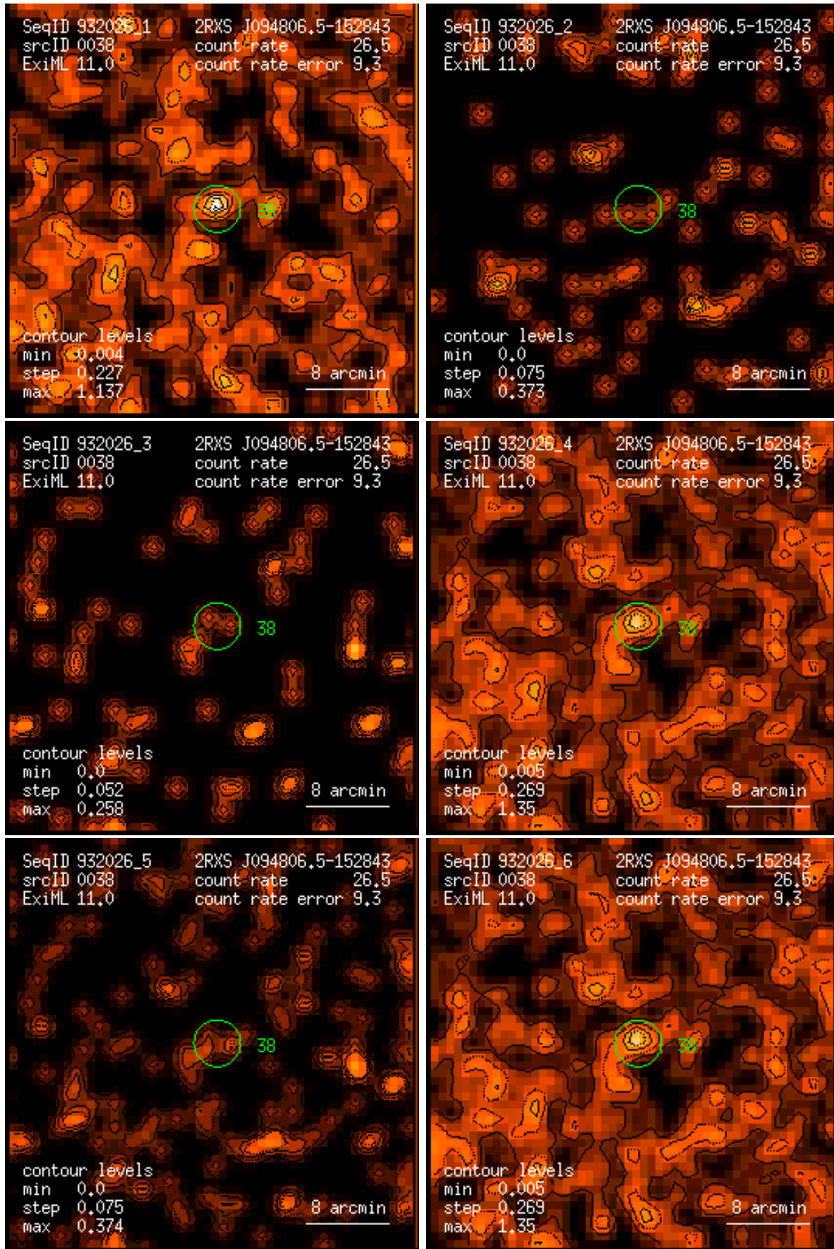
Figure 38: RASS 932026: detection 0038: band rate images, Gaussian filter: (1) PSPC channels 11 – 41, (2) 52 – 90, (3) 91 – 201, (4) 11 – 235, (5) 52 – 201, (6) 11 – 201. Broad band rates in counts/ks. Band rate contour levels in counts/ks/arcmin 2 .
