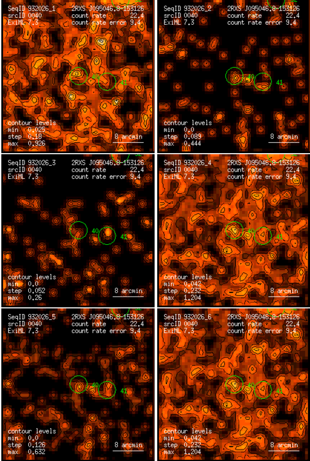
Figure 40: RASS 932026: detection 0040: band rate images, Gaussian filter: (1) PSPC channels 11 – 41, (2) 52 – 90, (3) 91 – 201, (4) 11 – 235, (5) 52 – 201, (6) 11 – 201. Broad band rates in counts/ks. Band rate contour levels in counts/ks/arcmin 2 .
