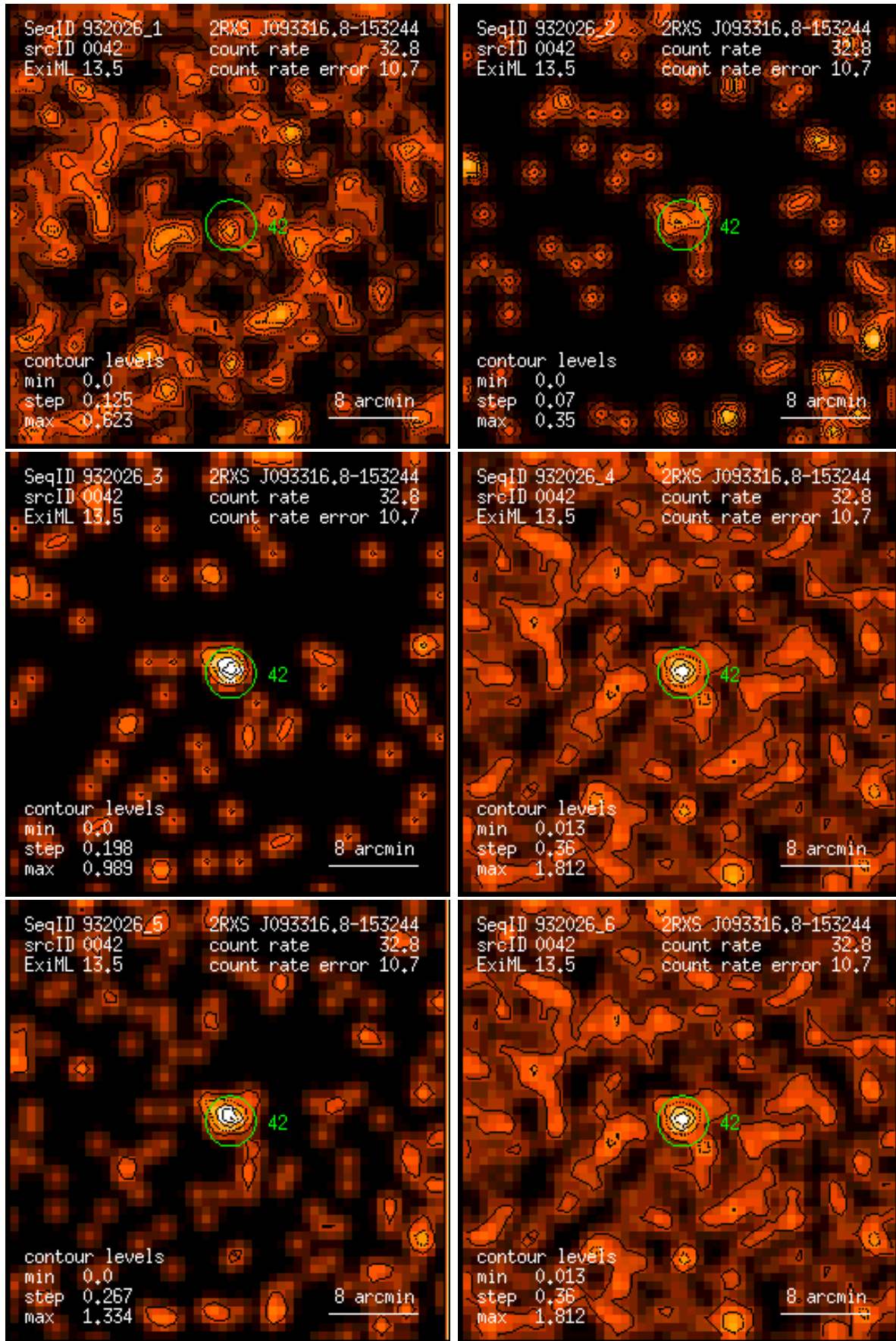
Figure 42: RASS 932026: detection 0042: band rate images, Gaussian filter: (1) PSPC channels 11 – 41, (2) 52 – 90, (3) 91 – 201, (4) 11 – 235, (5) 52 – 201, (6) 11 – 201. Broad band rates in counts/ks. Band rate contour levels in counts/ks/arcmin 2 .
