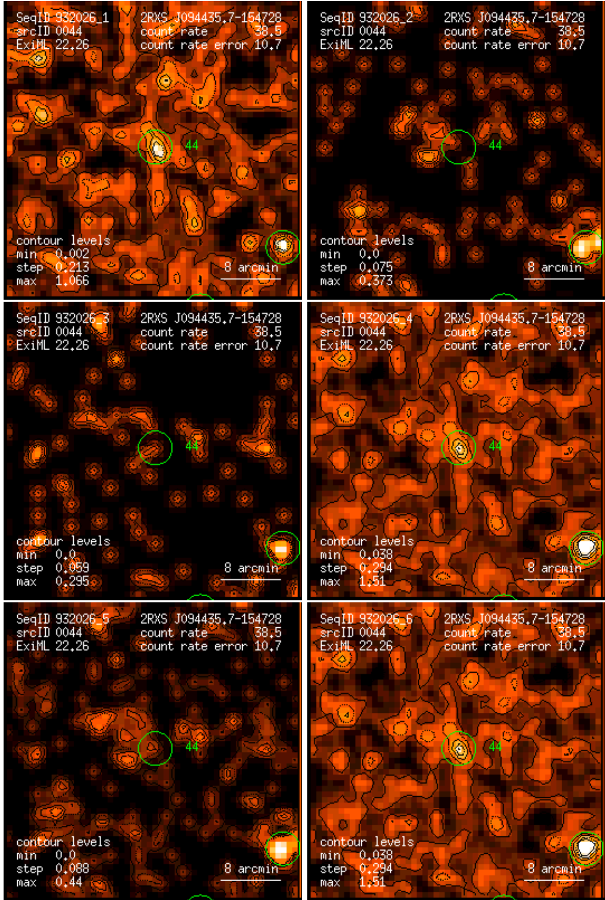
Figure 44: RASS 932026: detection 0044: band rate images, Gaussian filter: (1) PSPC channels 11 – 41, (2) 52 – 90, (3) 91 – 201, (4) 11 – 235, (5) 52 – 201, (6) 11 – 201. Broad band rates in counts/ks. Band rate contour levels in counts/ks/arcmin 2 .
