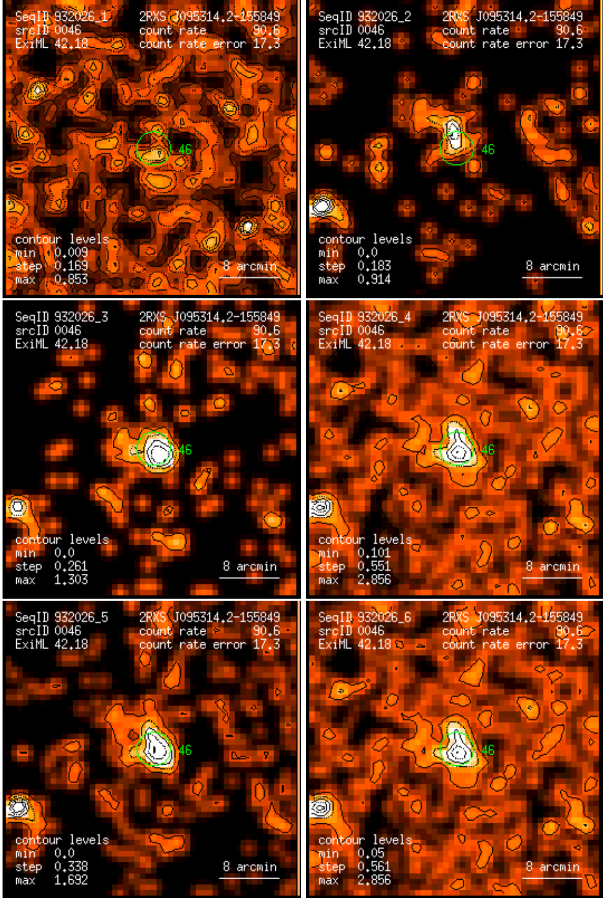
Figure 46: RASS 932026: detection 0046: band rate images, Gaussian filter: (1) PSPC channels 11 – 41, (2) 52 – 90, (3) 91 – 201, (4) 11 – 235, (5) 52 – 201, (6) 11 – 201. Broad band rates in counts/ks. Band rate contour levels in counts/ks/arcmin 2 .
