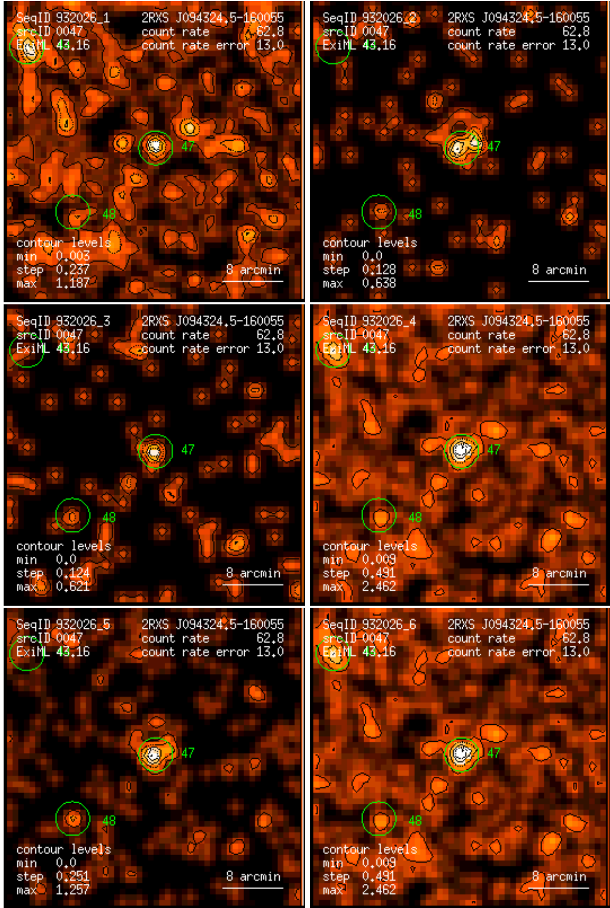
Figure 47: RASS 932026: detection 0047: band rate images, Gaussian filter: (1) PSPC channels 11 – 41, (2) 52 – 90, (3) 91 – 201, (4) 11 – 235, (5) 52 – 201, (6) 11 – 201. Broad band rates in counts/ks. Band rate contour levels in counts/ks/arcmin 2 .
