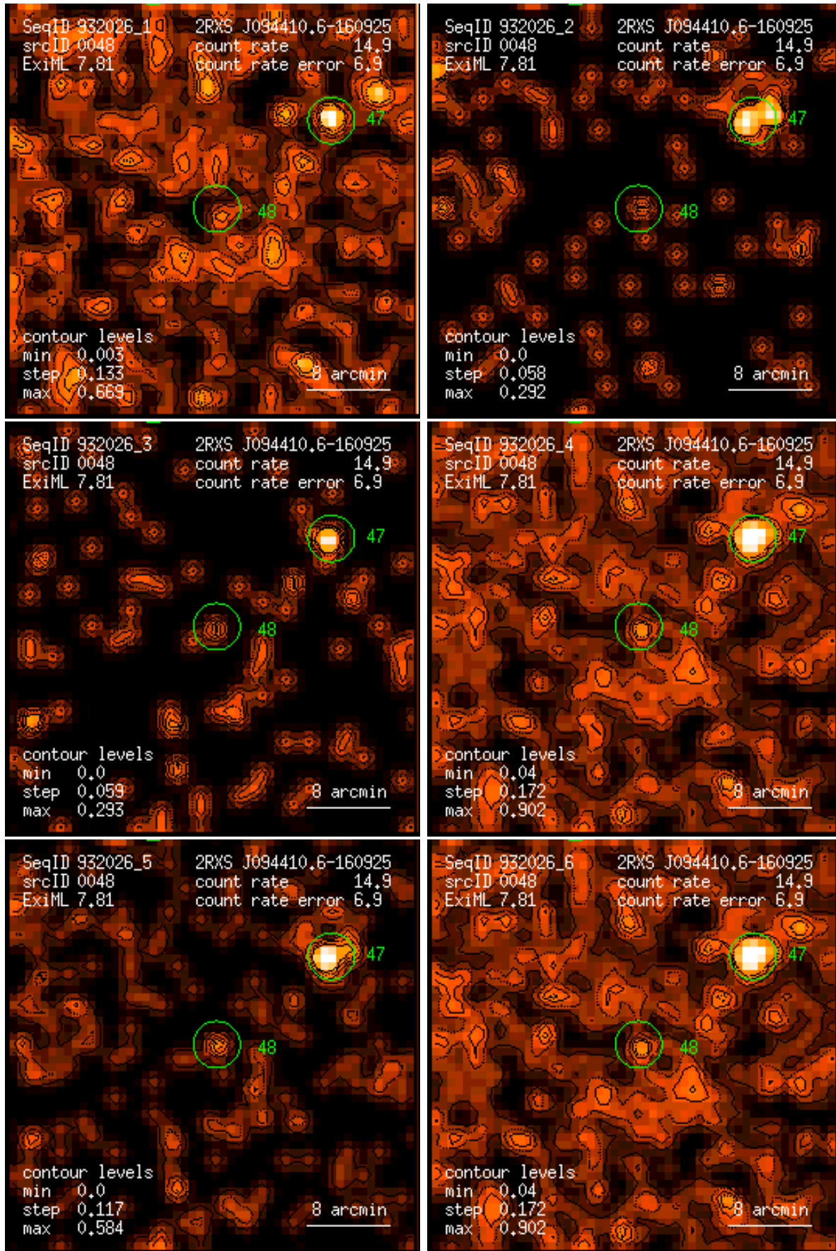
Figure 48: RASS 932026: detection 0048: band rate images, Gaussian filter: (1) PSPC channels 11 – 41, (2) 52 – 90, (3) 91 – 201, (4) 11 – 235, (5) 52 – 201, (6) 11 – 201. Broad band rates in counts/ks. Band rate contour levels in counts/ks/arcmin 2 .
