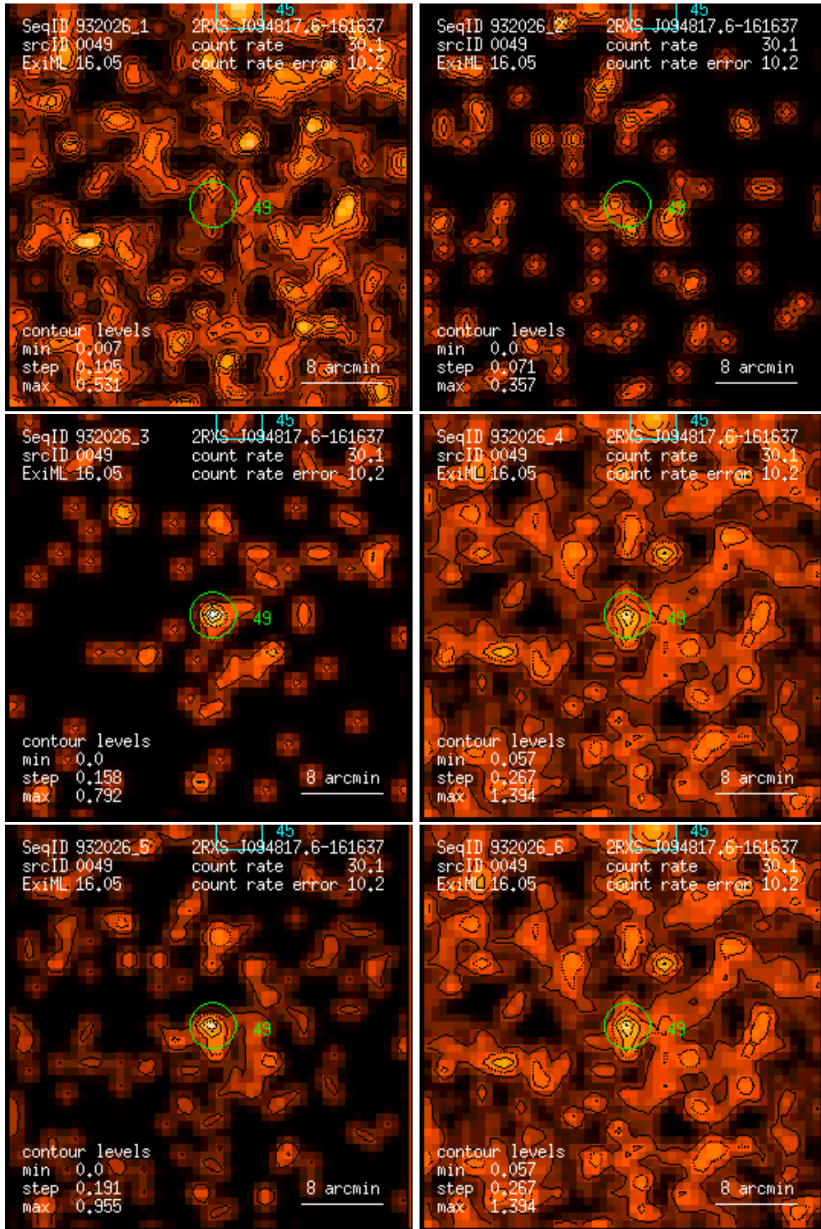
Figure 49: RASS 932026: detection 0049: band rate images, Gaussian filter: (1) PSPC channels 11 – 41, (2) 52 – 90, (3) 91 – 201, (4) 11 – 235, (5) 52 – 201, (6) 11 – 201. Broad band rates in counts/ks. Band rate contour levels in counts/ks/arcmin 2 .
