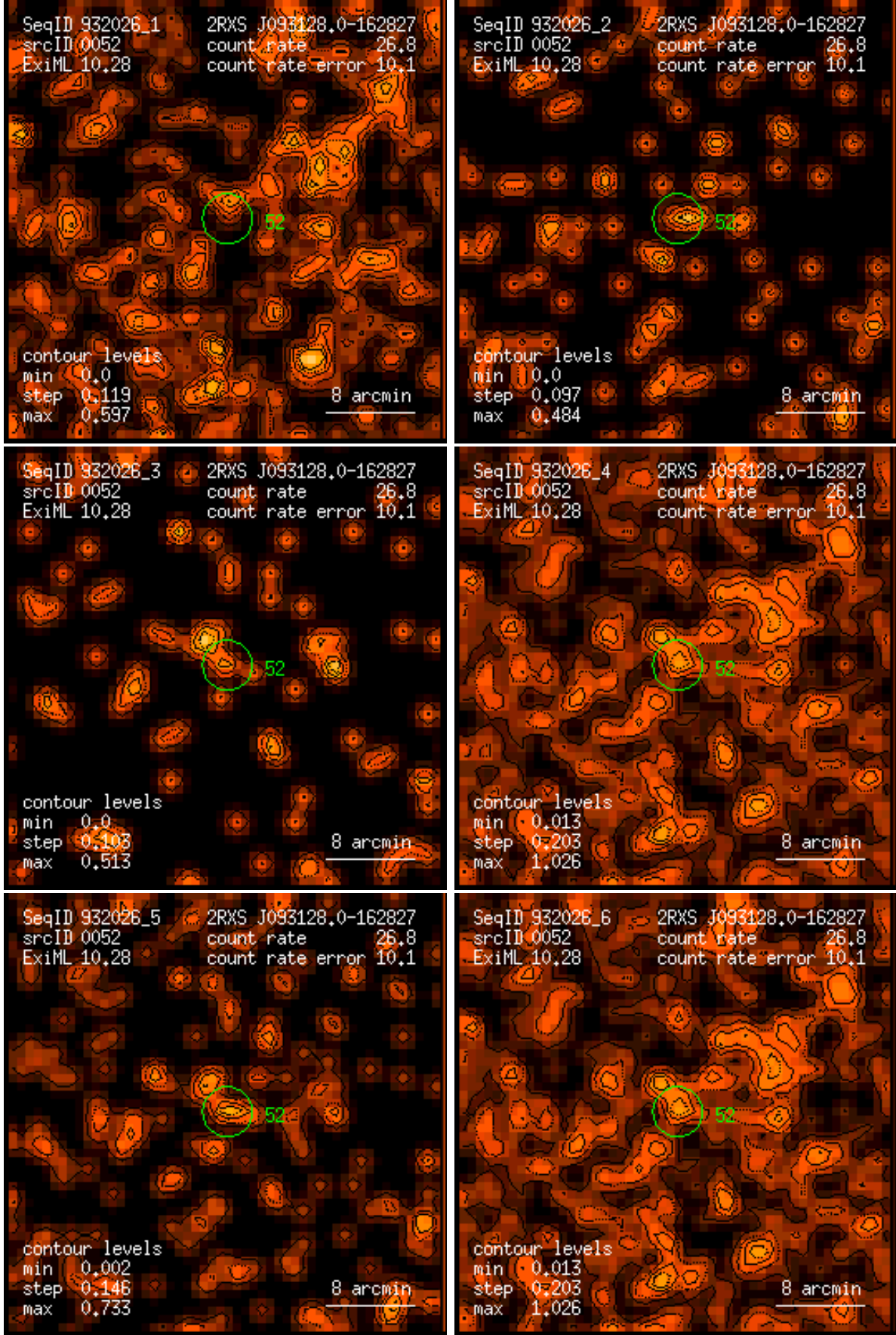
Figure 52: RASS 932026: detection 0052: band rate images, Gaussian filter: (1) PSPC channels 11 – 41, (2) 52 – 90, (3) 91 – 201, (4) 11 – 235, (5) 52 – 201, (6) 11 – 201. Broad band rates in counts/ks. Band rate contour levels in counts/ks/arcmin 2 .
