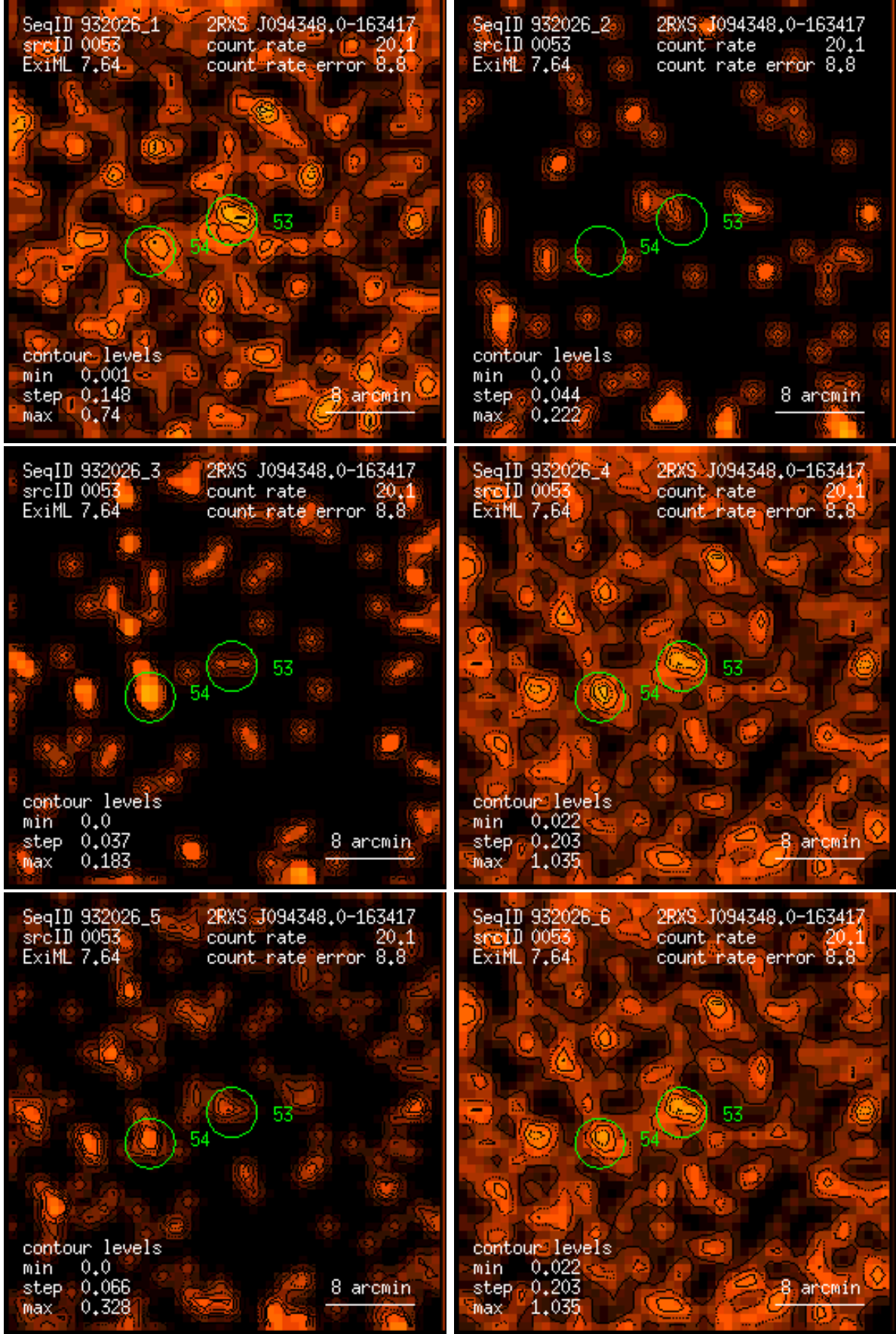
Figure 53: RASS 932026: detection 0053: band rate images, Gaussian filter: (1) PSPC channels 11 – 41, (2) 52 – 90, (3) 91 – 201, (4) 11 – 235, (5) 52 – 201, (6) 11 – 201. Broad band rates in counts/ks. Band rate contour levels in counts/ks/arcmin 2 .
