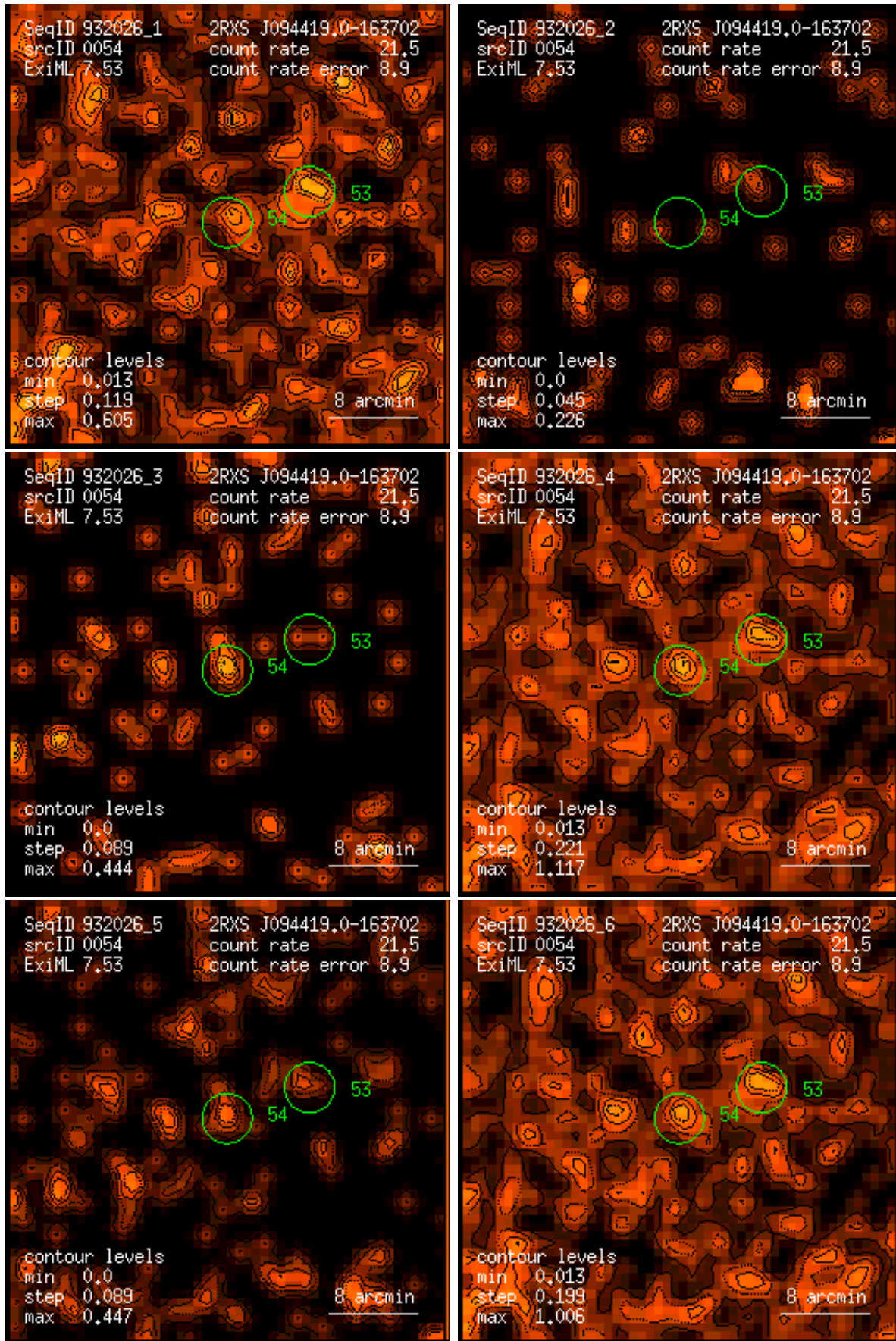
Figure 54: RASS 932026: detection 0054: band rate images, Gaussian filter: (1) PSPC channels 11 – 41, (2) 52 – 90, (3) 91 – 201, (4) 11 – 235, (5) 52 – 201, (6) 11 – 201. Broad band rates in counts/ks. Band rate contour levels in counts/ks/arcmin 2 .
