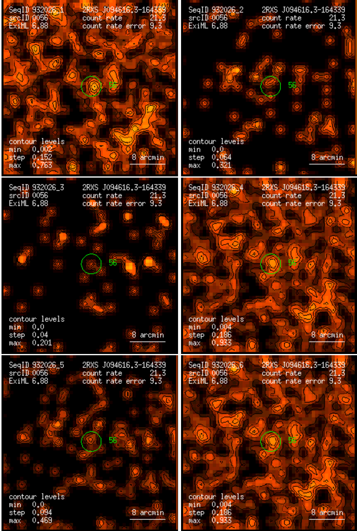
Figure 56: RASS 932026: detection 0056: band rate images, Gaussian filter: (1) PSPC channels 11 – 41, (2) 52 – 90, (3) 91 – 201, (4) 11 – 235, (5) 52 – 201, (6) 11 – 201. Broad band rates in counts/ks. Band rate contour levels in counts/ks/arcmin 2 .
