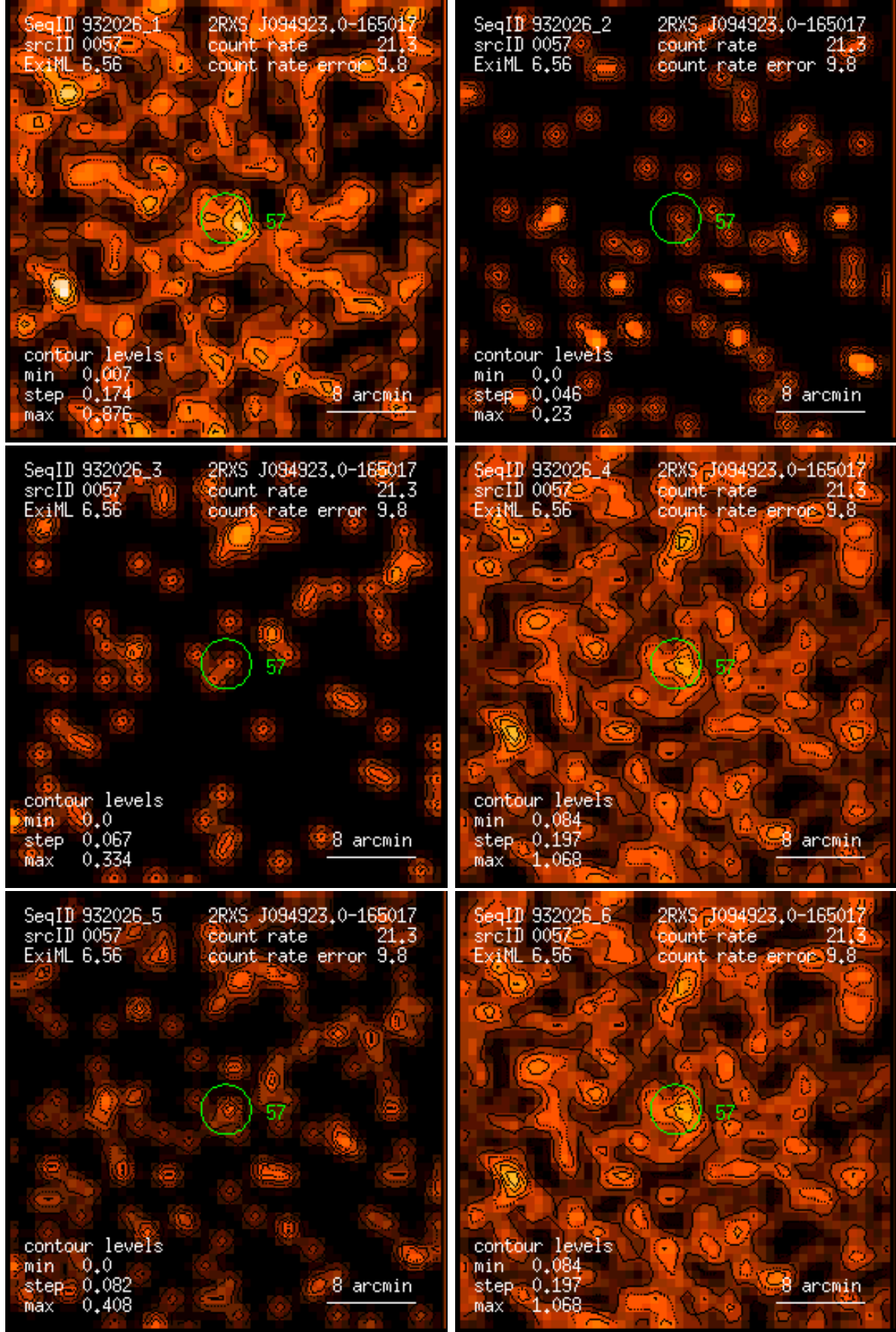
Figure 57: RASS 932026: detection 0057: band rate images, Gaussian filter: (1) PSPC channels 11 – 41, (2) 52 – 90, (3) 91 – 201, (4) 11 – 235, (5) 52 – 201, (6) 11 – 201. Broad band rates in counts/ks. Band rate contour levels in counts/ks/arcmin 2 .
