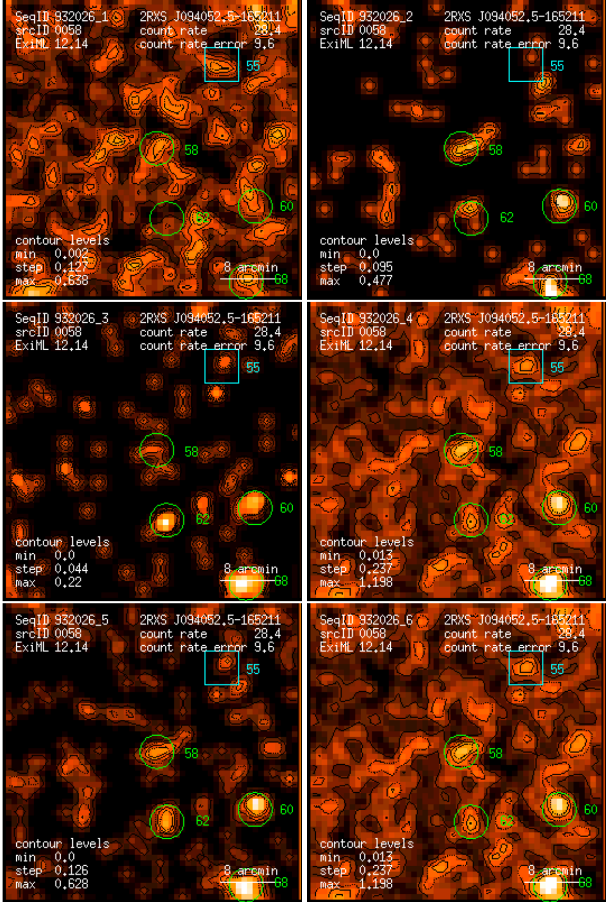
Figure 58: RASS 932026: detection 0058: band rate images, Gaussian filter: (1) PSPC channels 11 – 41, (2) 52 – 90, (3) 91 – 201, (4) 11 – 235, (5) 52 – 201, (6) 11 – 201. Broad band rates in counts/ks. Band rate contour levels in counts/ks/arcmin 2 .
