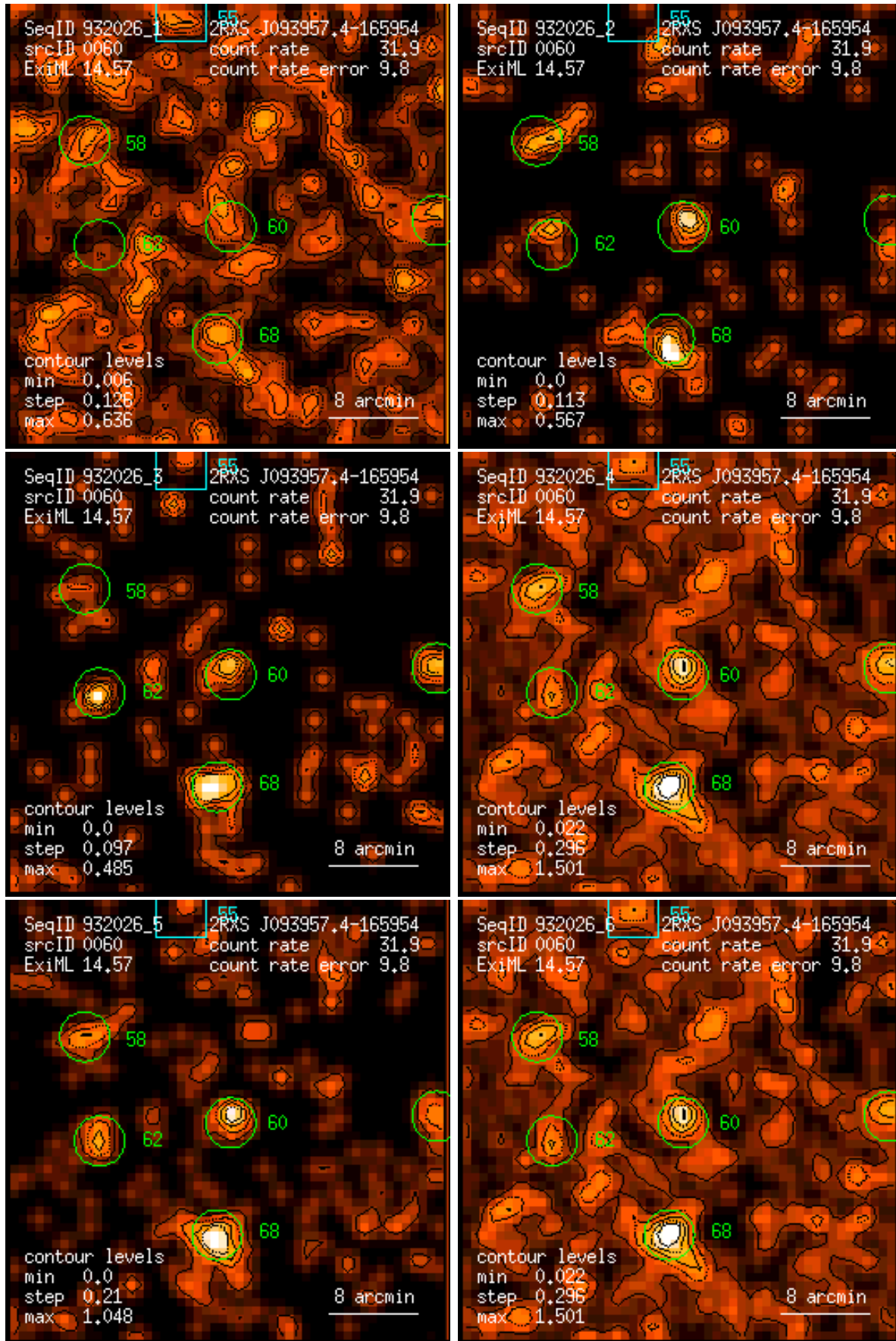
Figure 60: RASS 932026: detection 0060: band rate images, Gaussian filter: (1) PSPC channels 11 – 41, (2) 52 – 90, (3) 91 – 201, (4) 11 – 235, (5) 52 – 201, (6) 11 – 201. Broad band rates in counts/ks. Band rate contour levels in counts/ks/arcmin 2 .
