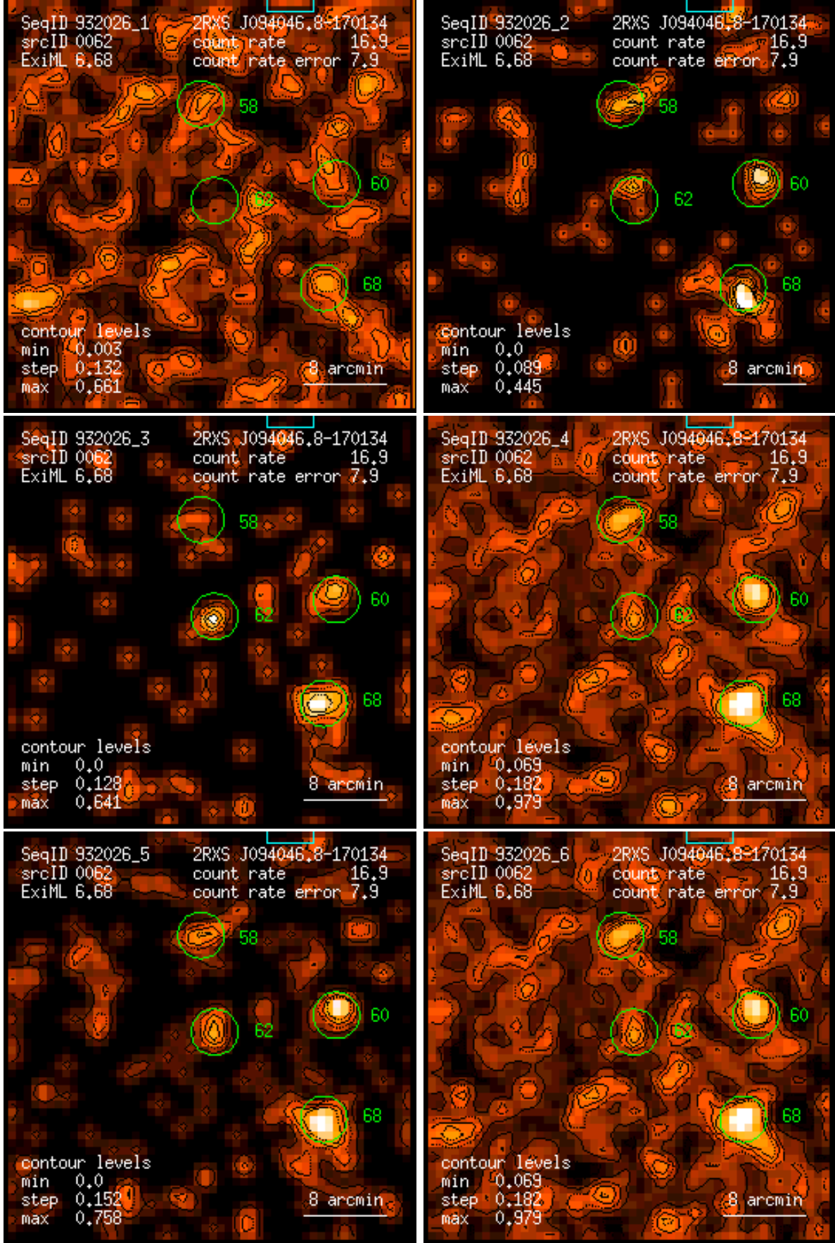
Figure 62: RASS 932026: detection 0062: band rate images, Gaussian filter: (1) PSPC channels 11 – 41, (2) 52 – 90, (3) 91 – 201, (4) 11 – 235, (5) 52 – 201, (6) 11 – 201. Broad band rates in counts/ks. Band rate contour levels in counts/ks/arcmin 2 .
