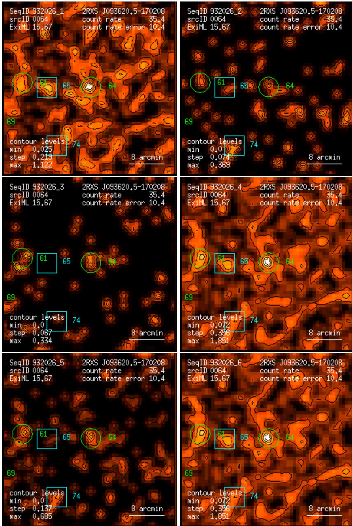
Figure 64: RASS 932026: detection 0064: band rate images, Gaussian filter: (1) PSPC channels 11 – 41, (2) 52 – 90, (3) 91 – 201, (4) 11 – 235, (5) 52 – 201, (6) 11 – 201. Broad band rates in counts/ks. Band rate contour levels in counts/ks/arcmin 2 .
