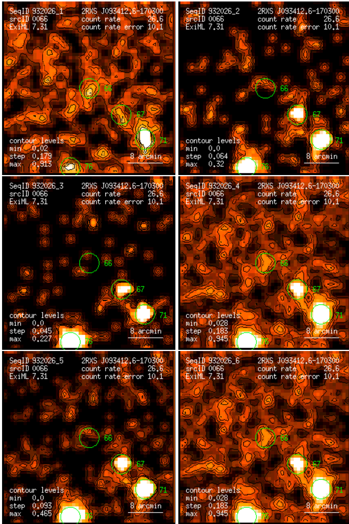
Figure 66: RASS 932026: detection 0066: band rate images, Gaussian filter: (1) PSPC channels 11 – 41, (2) 52 – 90, (3) 91 – 201, (4) 11 – 235, (5) 52 – 201, (6) 11 – 201. Broad band rates in counts/ks. Band rate contour levels in counts/ks/arcmin 2 .
