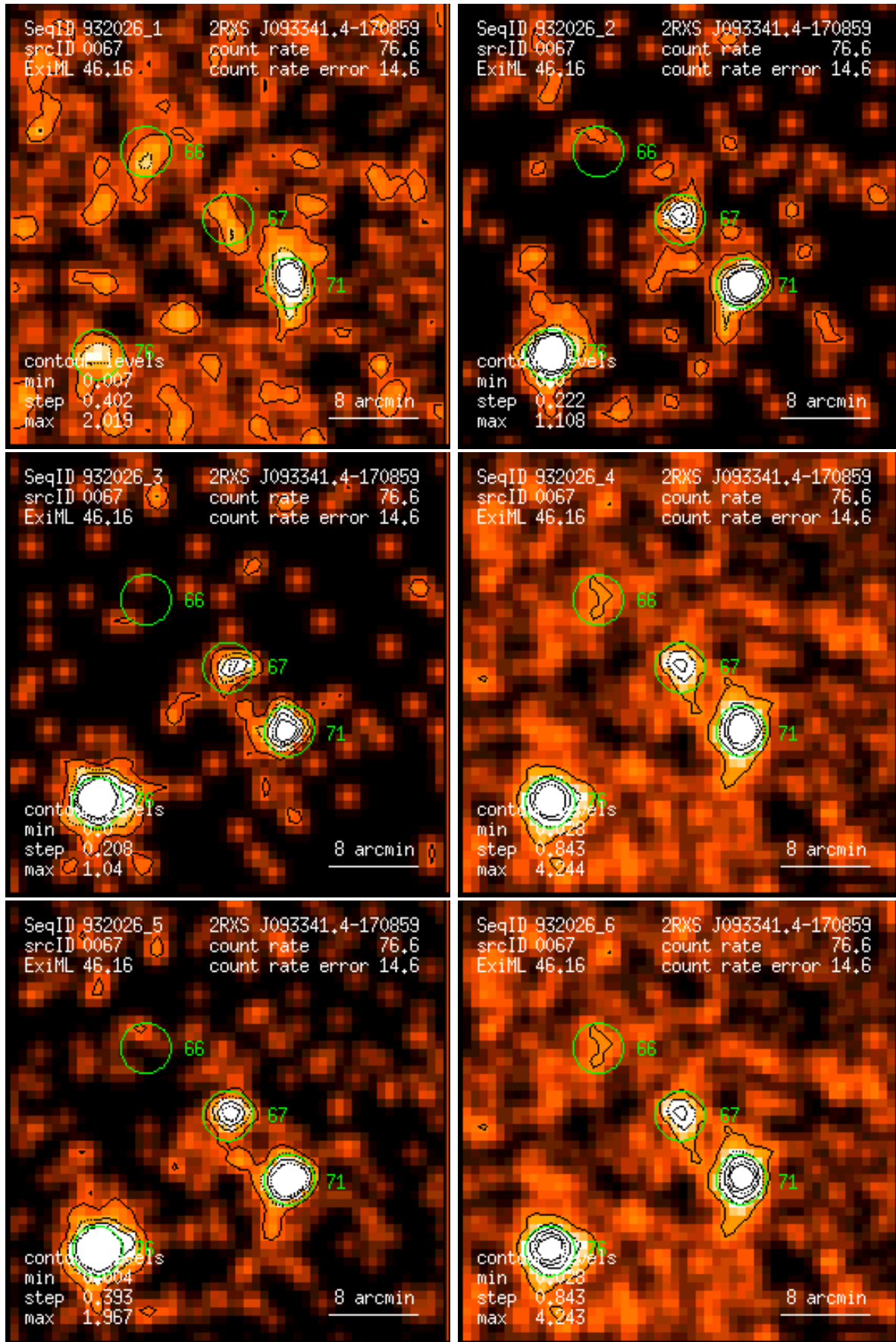
Figure 67: RASS 932026: detection 0067: band rate images, Gaussian filter: (1) PSPC channels 11 – 41, (2) 52 – 90, (3) 91 – 201, (4) 11 – 235, (5) 52 – 201, (6) 11 – 201. Broad band rates in counts/ks. Band rate contour levels in counts/ks/arcmin 2 .
