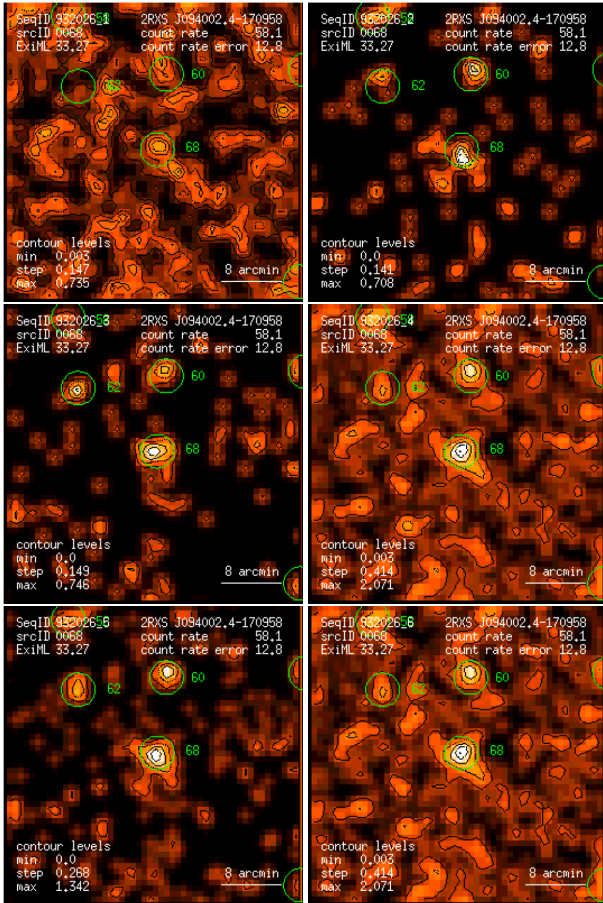
Figure 68: RASS 932026: detection 0068: band rate images, Gaussian filter: (1) PSPC channels 11 – 41, (2) 52 – 90, (3) 91 – 201, (4) 11 – 235, (5) 52 – 201, (6) 11 – 201. Broad band rates in counts/ks. Band rate contour levels in counts/ks/arcmin 2 .
