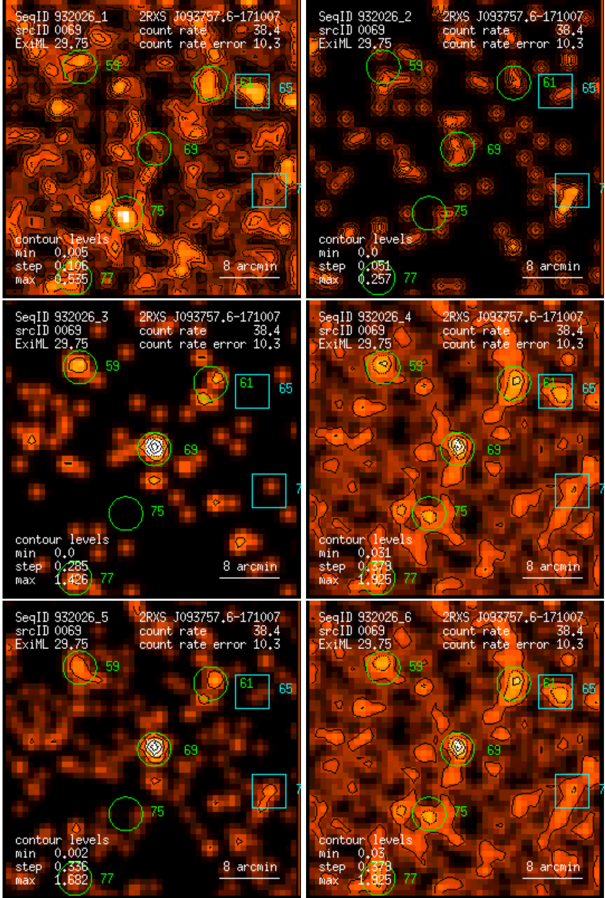
Figure 69: RASS 932026: detection 0069: band rate images, Gaussian filter: (1) PSPC channels 11 – 41, (2) 52 – 90, (3) 91 – 201, (4) 11 – 235, (5) 52 – 201, (6) 11 – 201. Broad band rates in counts/ks. Band rate contour levels in counts/ks/arcmin 2 .
