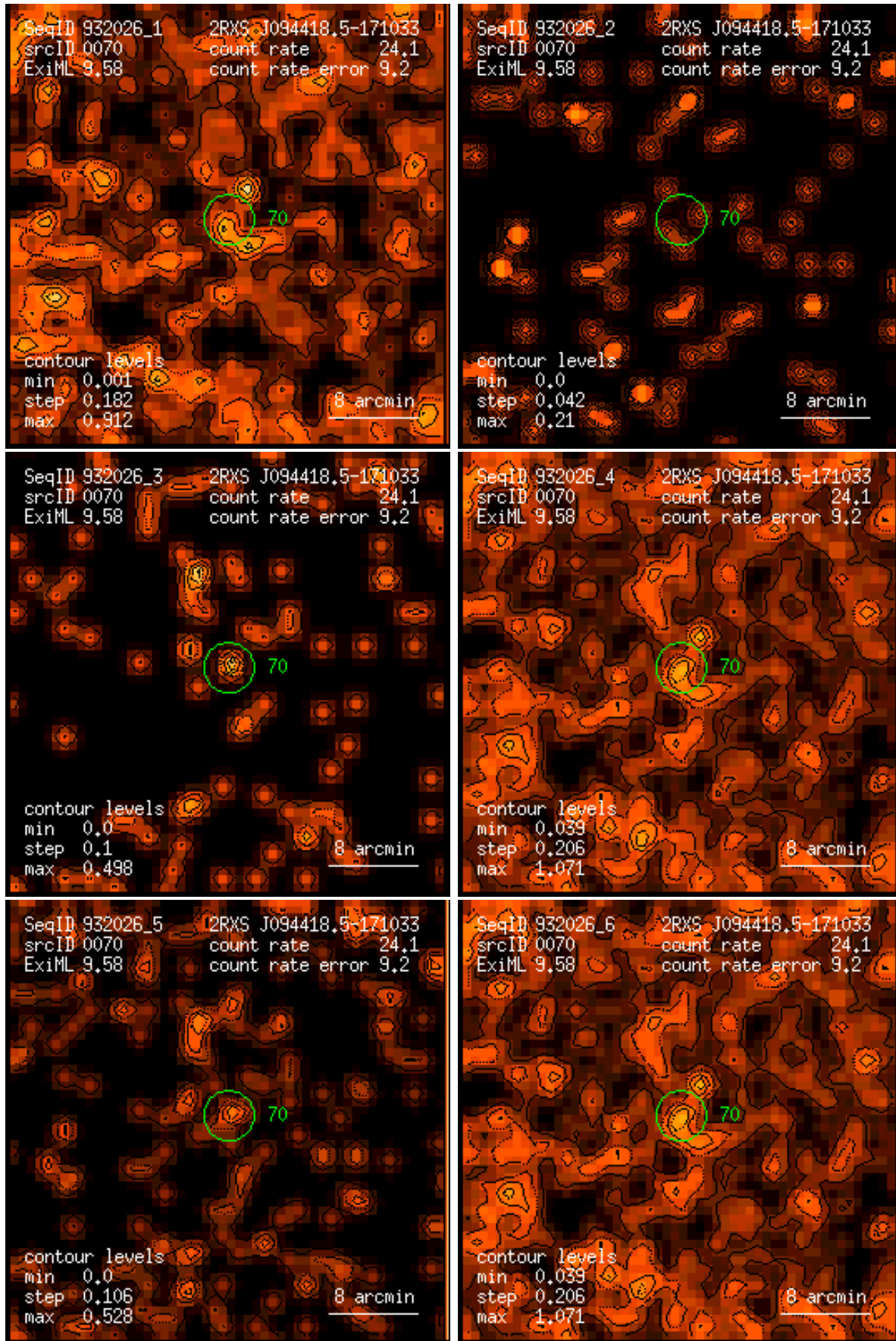
Figure 70: RASS 932026: detection 0070: band rate images, Gaussian filter: (1) PSPC channels 11 – 41, (2) 52 – 90, (3) 91 – 201, (4) 11 – 235, (5) 52 – 201, (6) 11 – 201. Broad band rates in counts/ks. Band rate contour levels in counts/ks/arcmin 2 .
