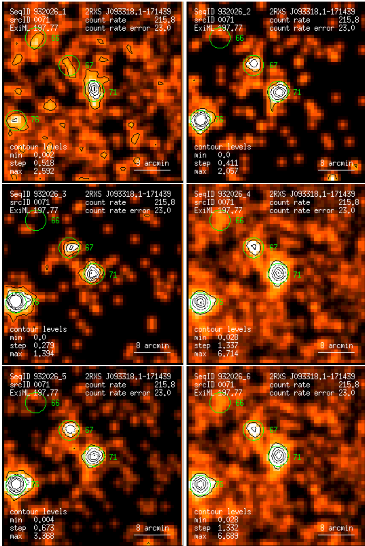
Figure 71: RASS 932026: detection 0071: band rate images, Gaussian filter: (1) PSPC channels 11 – 41, (2) 52 – 90, (3) 91 – 201, (4) 11 – 235, (5) 52 – 201, (6) 11 – 201. Broad band rates in counts/ks. Band rate contour levels in counts/ks/arcmin 2 .
