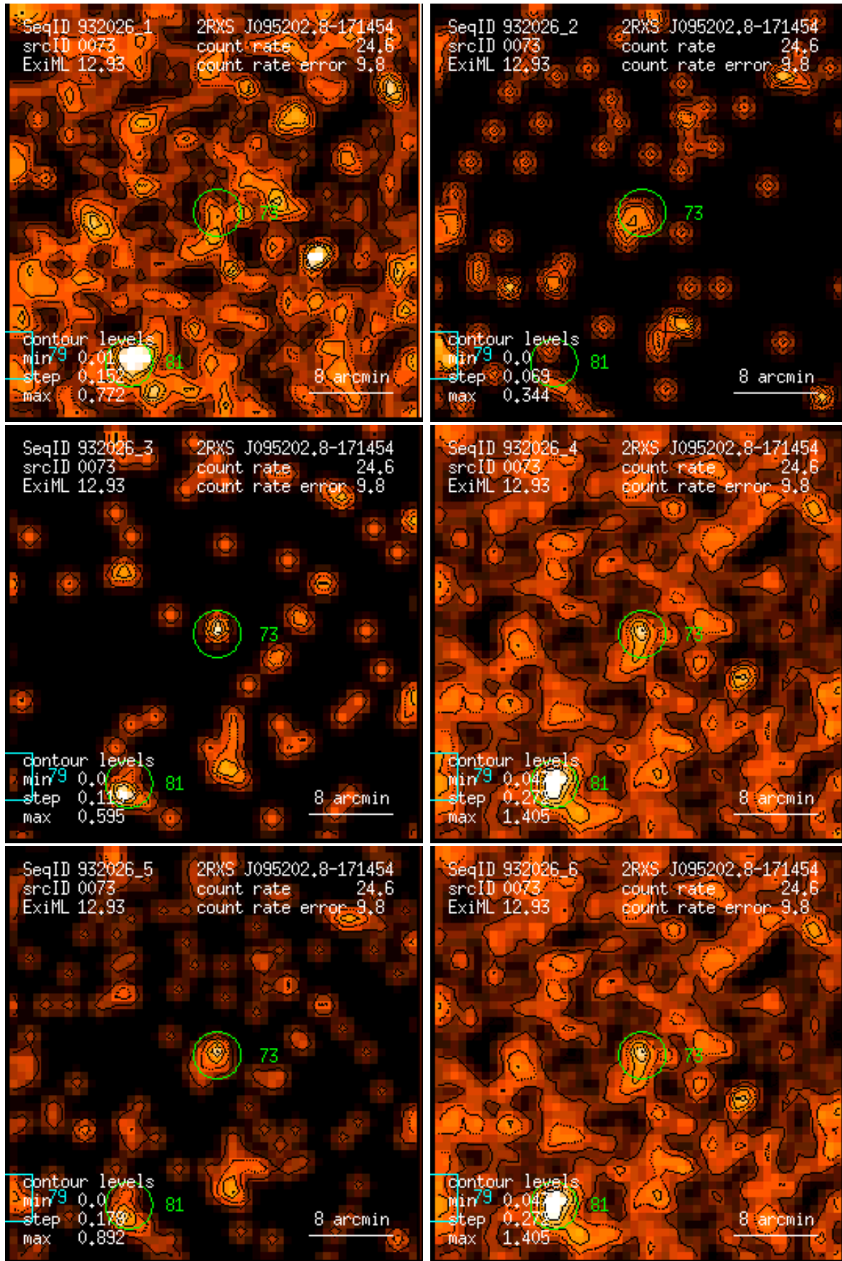
Figure 73: RASS 932026: detection 0073: band rate images, Gaussian filter: (1) PSPC channels 11 – 41, (2) 52 – 90, (3) 91 – 201, (4) 11 – 235, (5) 52 – 201, (6) 11 – 201. Broad band rates in counts/ks. Band rate contour levels in counts/ks/arcmin 2 .
