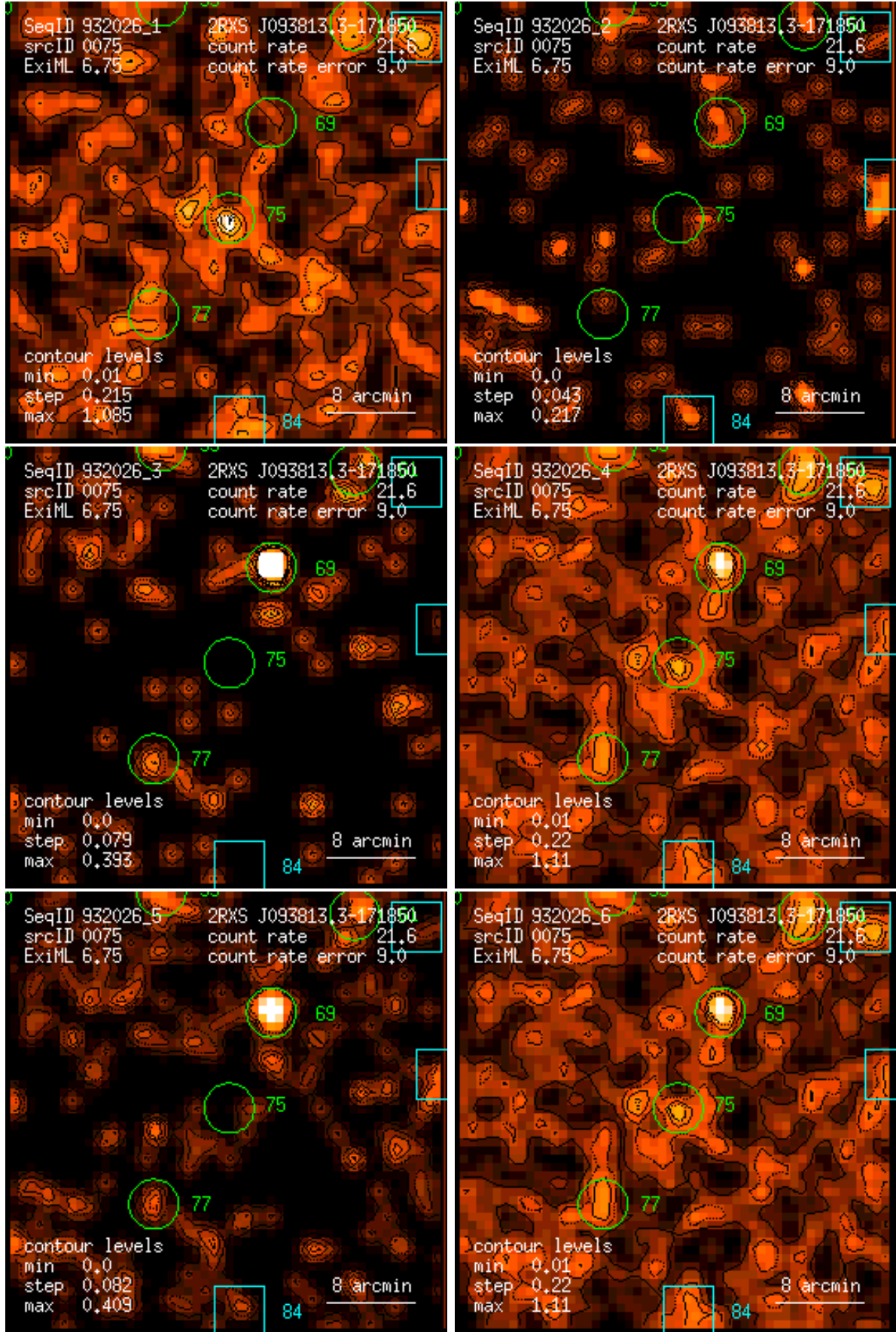
Figure 75: RASS 932026: detection 0075: band rate images, Gaussian filter: (1) PSPC channels 11 – 41, (2) 52 – 90, (3) 91 – 201, (4) 11 – 235, (5) 52 – 201, (6) 11 – 201. Broad band rates in counts/ks. Band rate contour levels in counts/ks/arcmin 2 .
