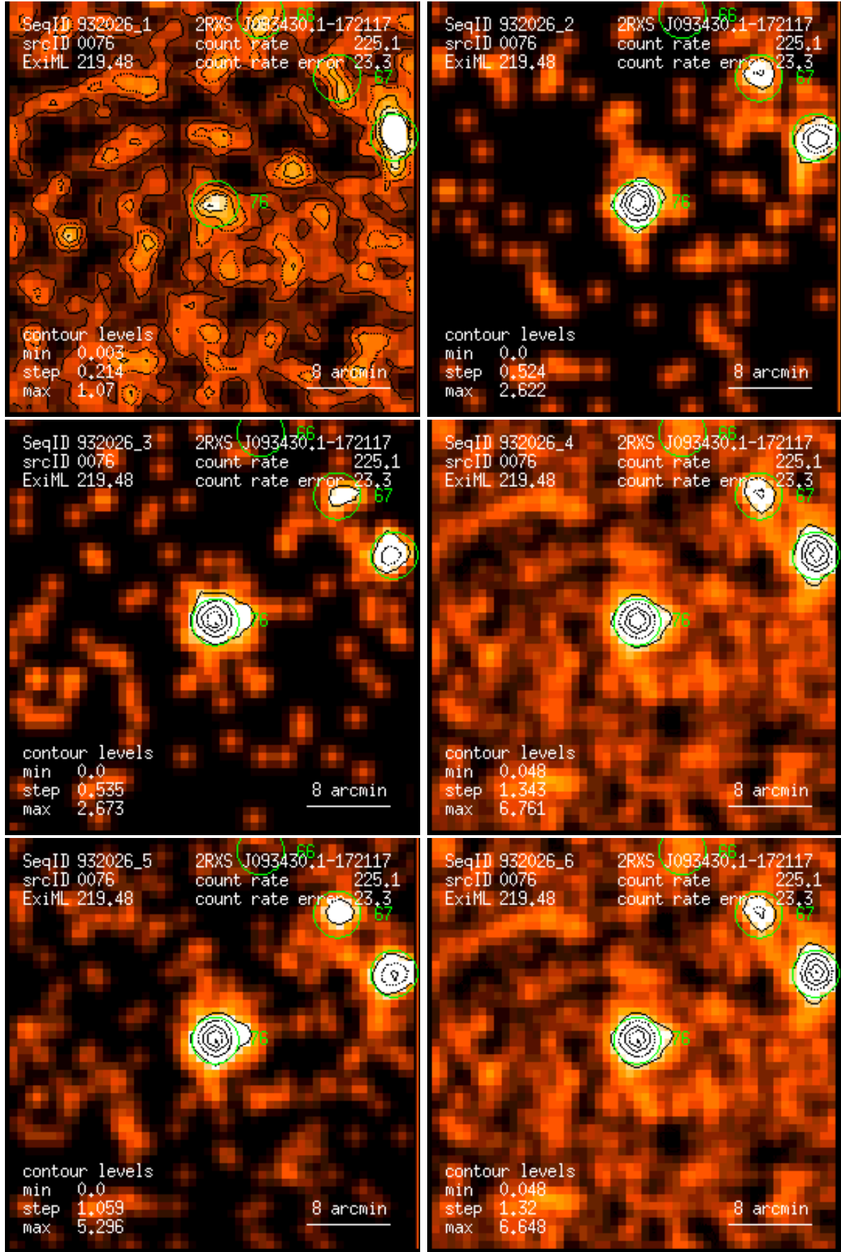
Figure 76: RASS 932026: detection 0076: band rate images, Gaussian filter: (1) PSPC channels 11 – 41, (2) 52 – 90, (3) 91 – 201, (4) 11 – 235, (5) 52 – 201, (6) 11 – 201. Broad band rates in counts/ks. Band rate contour levels in counts/ks/arcmin 2 .
