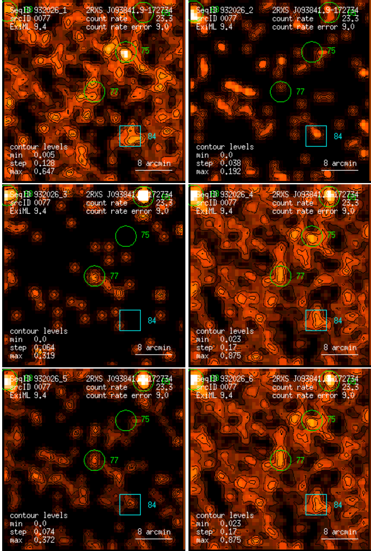
Figure 77: RASS 932026: detection 0077: band rate images, Gaussian filter: (1) PSPC channels 11 – 41, (2) 52 – 90, (3) 91 – 201, (4) 11 – 235, (5) 52 – 201, (6) 11 – 201. Broad band rates in counts/ks. Band rate contour levels in counts/ks/arcmin 2 .
